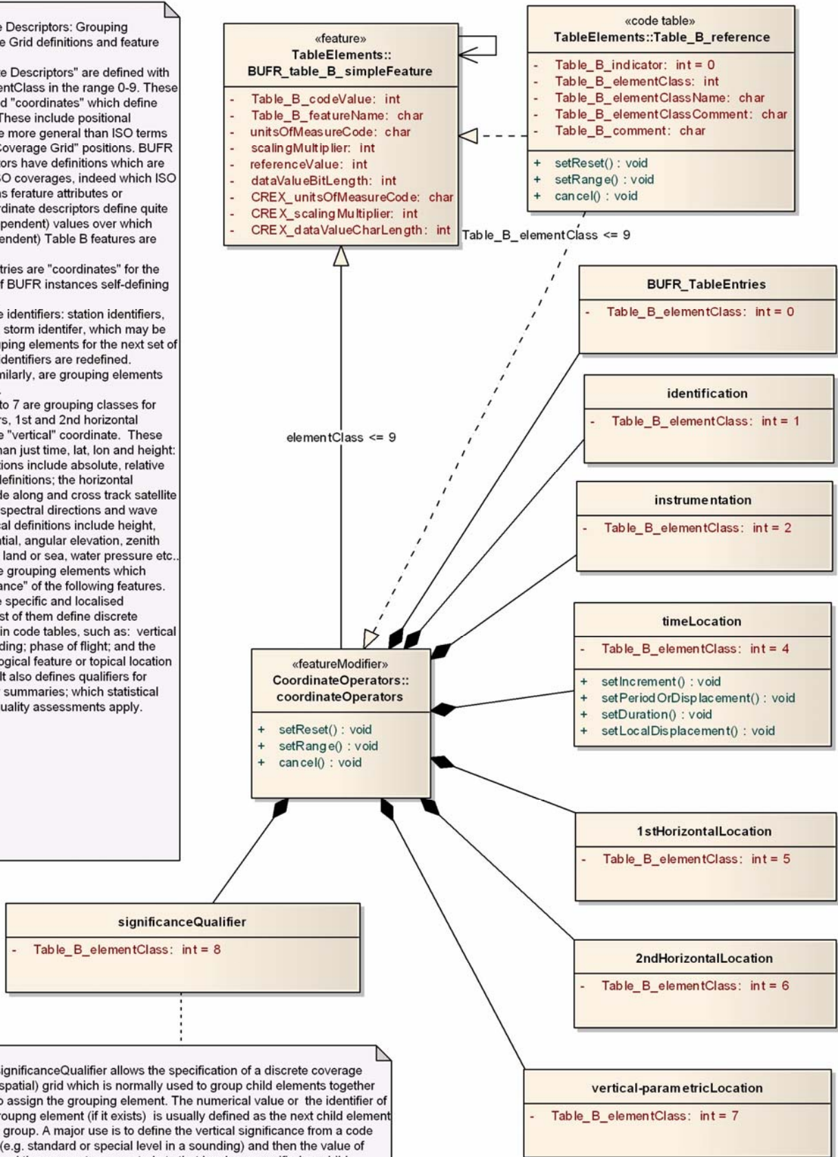
Figure 4: BUFR generalised "coordinates". CoordinateOperators modify features. They are grouping structures, coverage grid specifications and feature attribute definitions.
