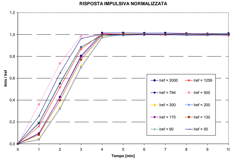
Figure 1: Sample step response determination for a weighing rain gauge with a time constant larger than one minute at various equivalent reference intensities.
