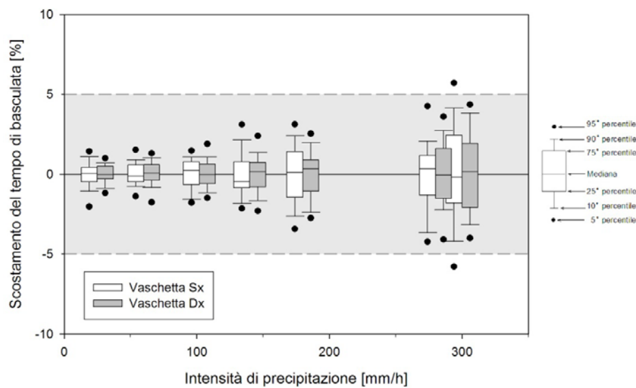
Figure III.1: Example of the non-parametric analysis of relative deviations from the average of the times of tipping of the left (Sx) and right (Dx) bucket for a well balanced instrument, where the 80% of the values is well within the \pm 5\% limits, over the entire operational range of measurement of the instrument.
