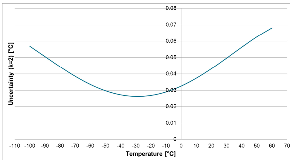
Figure 4. The calibration uncertainty of RS41 temperature measurement ( k=2 ).
