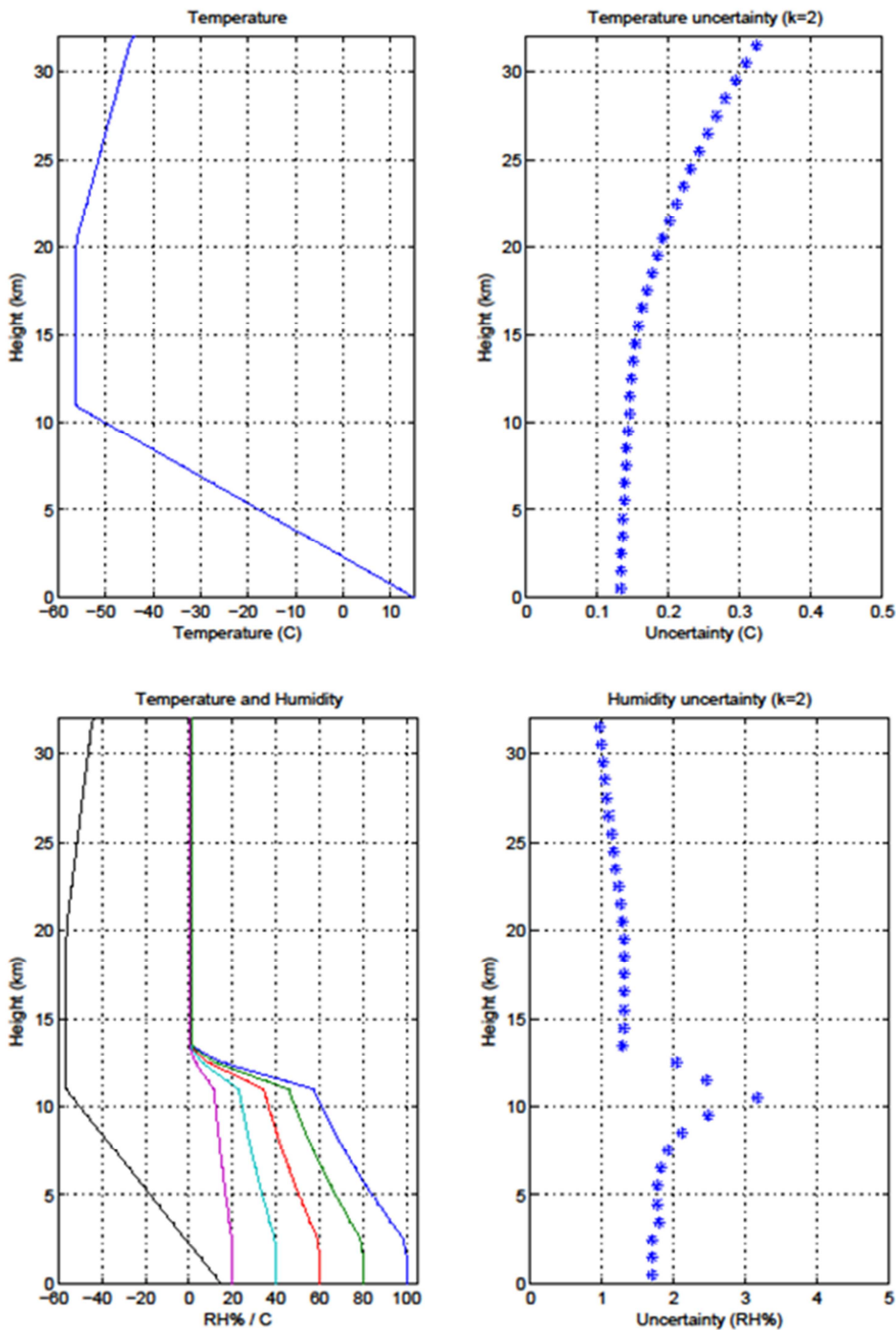
Figure 13. Top: The combined measurement uncertainty of RS41 temperature measurement ( k=2 ). The U.S. Standard Atmosphere 1976 temperature profile used in the uncertainty analysis (left) and the resulting temperature measurement uncertainty (right). Bottom: The combined measurement uncertainty of RS41 humidity measurement ( k=2 ). The uncertainty analysis model applied the U.S. Standard Atmosphere 1976 temperature profile and a set of humidity profiles (left), and the resulting humidity measurement uncertainty (right).
