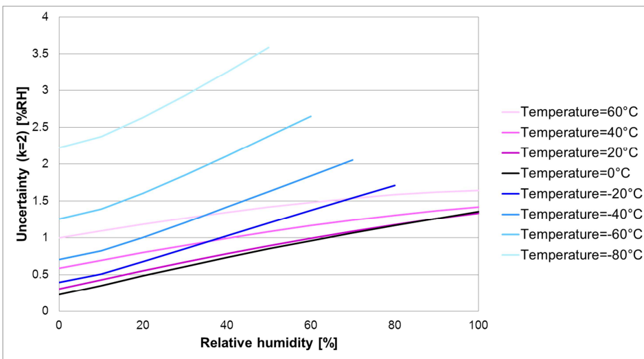
Figure 6. The combined calibration uncertainty (k=2) of RS41 humidity measurement including uncertainty components of temperature measurements and sensor model.
