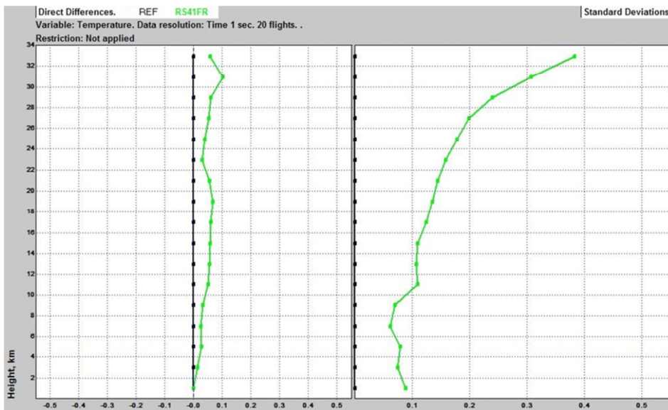
Figure 17. A twin-sounding comparison of RS41 temperature measurement against a multi-thermometer reference instrument – average temperature difference (left) and standard deviation of differences (right).
