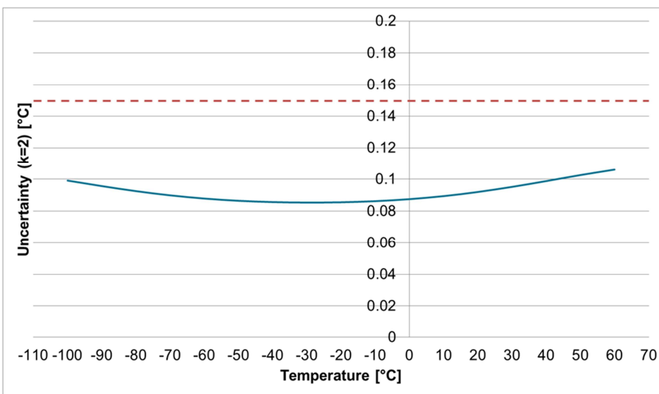
Figure 9. The combined uncertainty of the Vaisala Radiosonde RS41 temperature measurement after ground preparation (k=2). The dashed line indicates the calibration accuracy of RS92.
