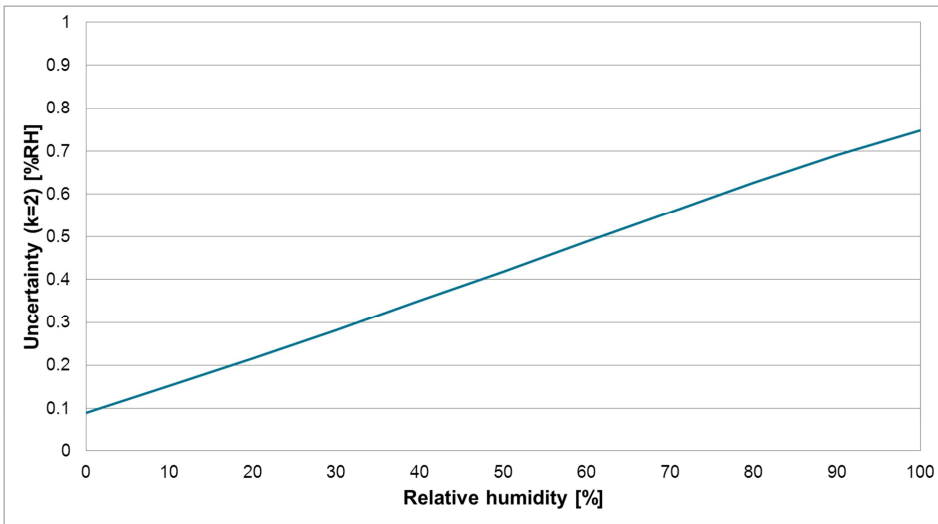
Figure 5. The calibration uncertainty of RS41 humidity measurement (k=2).
