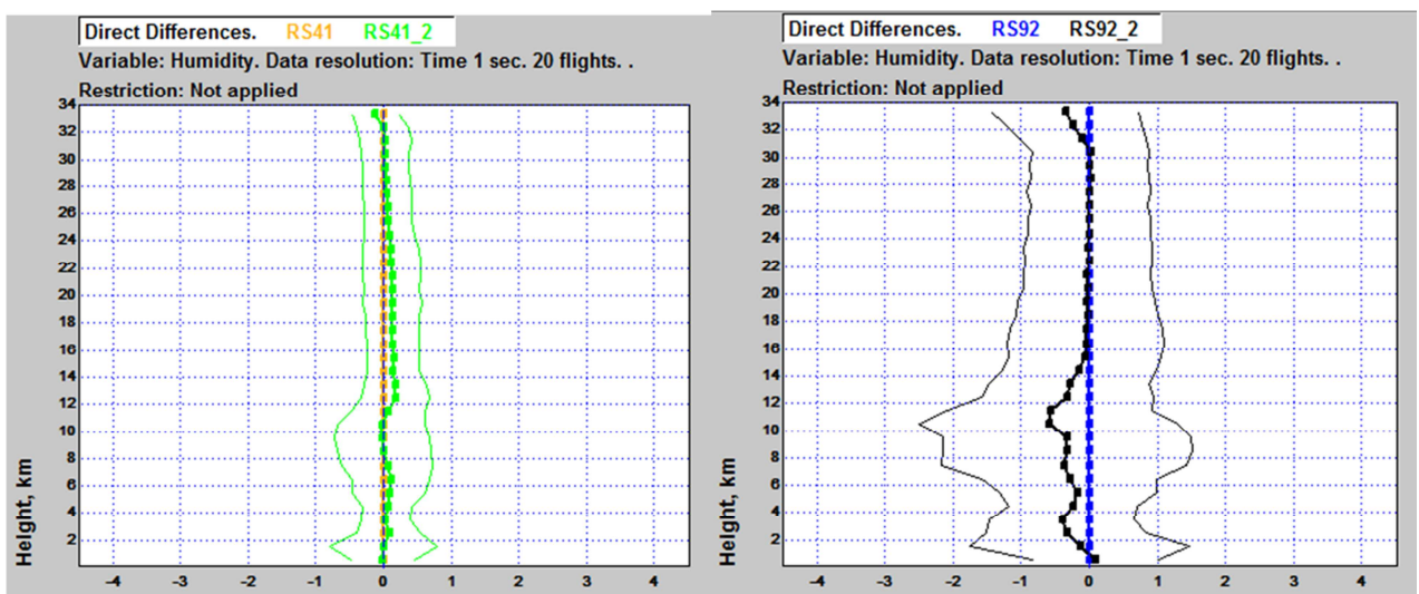
Figure 16. Reproducibility of daytime humidity measurement in Camborne campaign, RS41 on the left, RS92 on the right.
