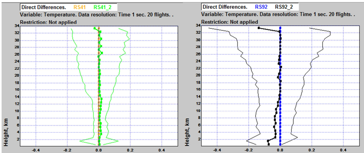
Figure 15. Reproducibility of daytime temperature measurement in Camborne campaign, RS41 on the left, RS92 on the right.
