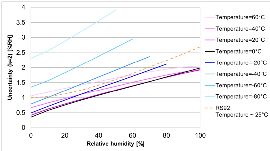
Figure 12. The combined uncertainty of Vaisala Radiosonde RS41 humidity measurement after ground preparation ( k=2 ) for various ambient temperatures. The dashed line indicates the corresponding RS92 uncertainty (lower limit) at room temperature derived in GRUAN data processing.
