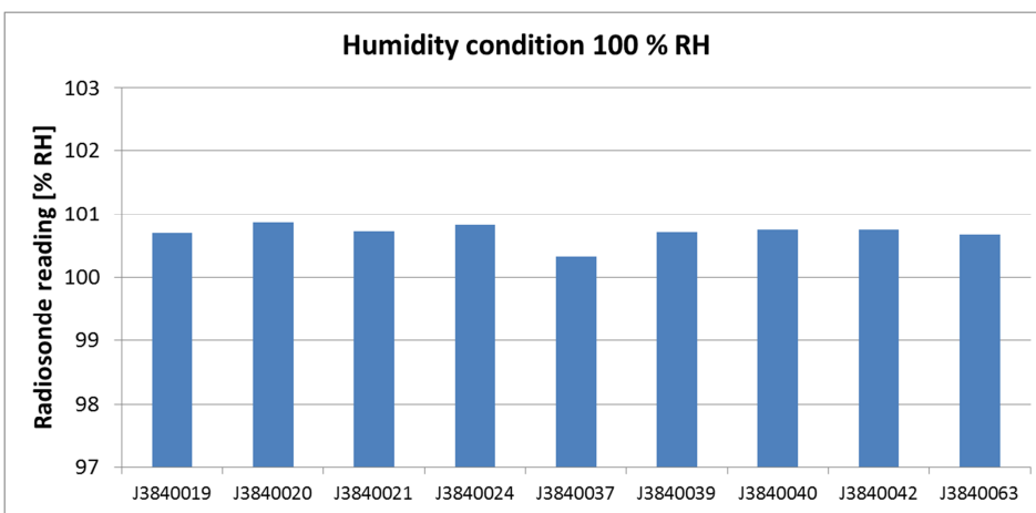
Figure 11. Stability test results after a six month storage, measurements in saturated humidity, temperature approximately 30°C.
