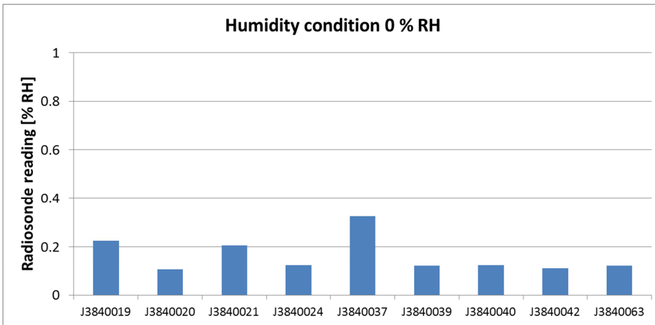
Figure 10. Stability test results after a six month storage, measurements in dry condition at room temperature.
