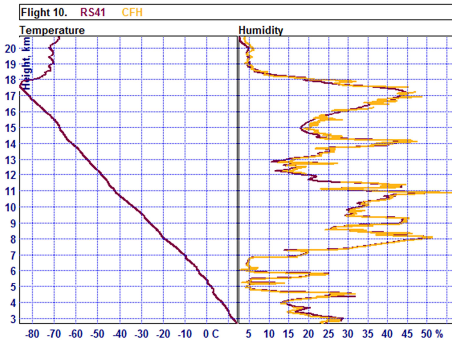
Figure 18. An example of a sounding carried out in Penang, Malaysia in 2013, compared against a CFH reference measurement. The figure shows relative humidity as measured by CFH (yellow) and the RS41 (brown).
