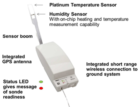
Figure 1. Design overview of RS41.
