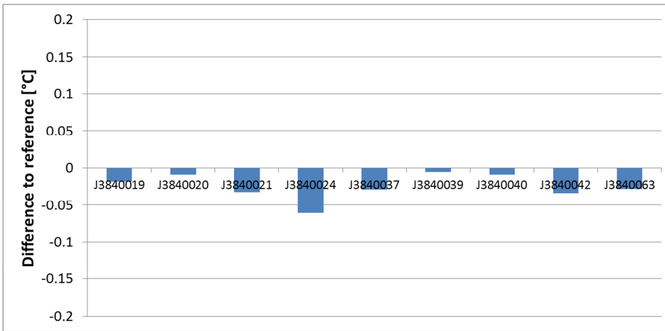
Figure 8. Stability test results after a six month storage, measurements at 20°C, test uncertainty 0.07°C (k=2).
