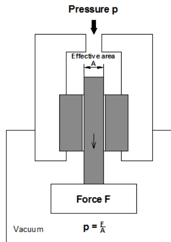
Figure 3.1. Piston gauge with dynamometer
