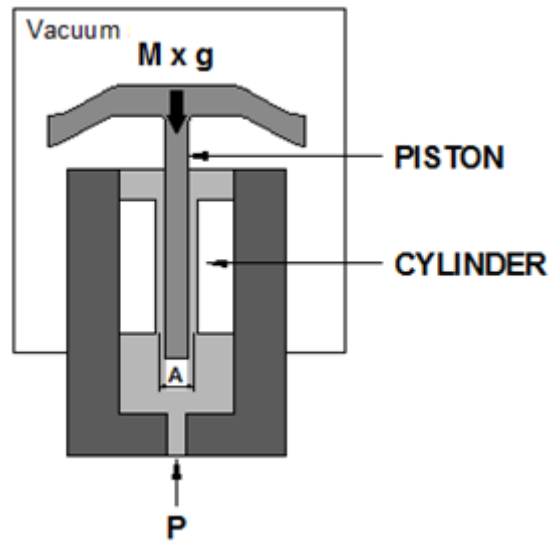
Figure 3.2. Loaded piston gauge
