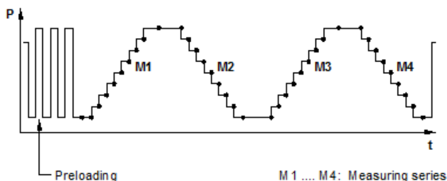
Figure 3.3. Calibration procedure
