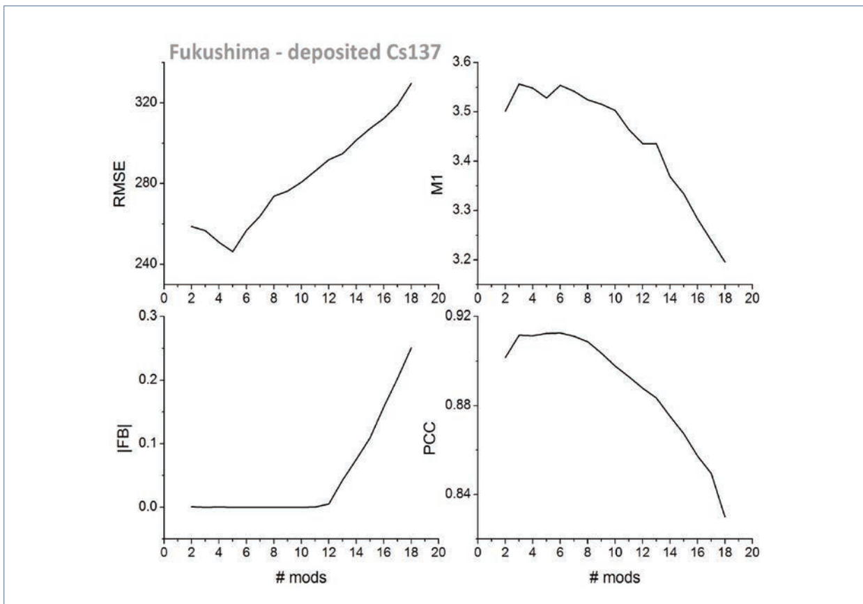
Figure 14. Clockwise from top left curves of minimum RMSE, maximum M1, maximum PCC, minimum FB, as a function of the number of models.
