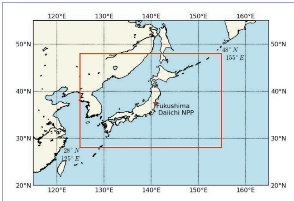
Figure 3. Regional domain (red box) over which task team calculations were performed.
