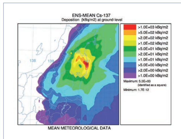
Figure 8. Calculated Cs-137 deposition using the mean of selected ten ATDM-meteorology combinations.
