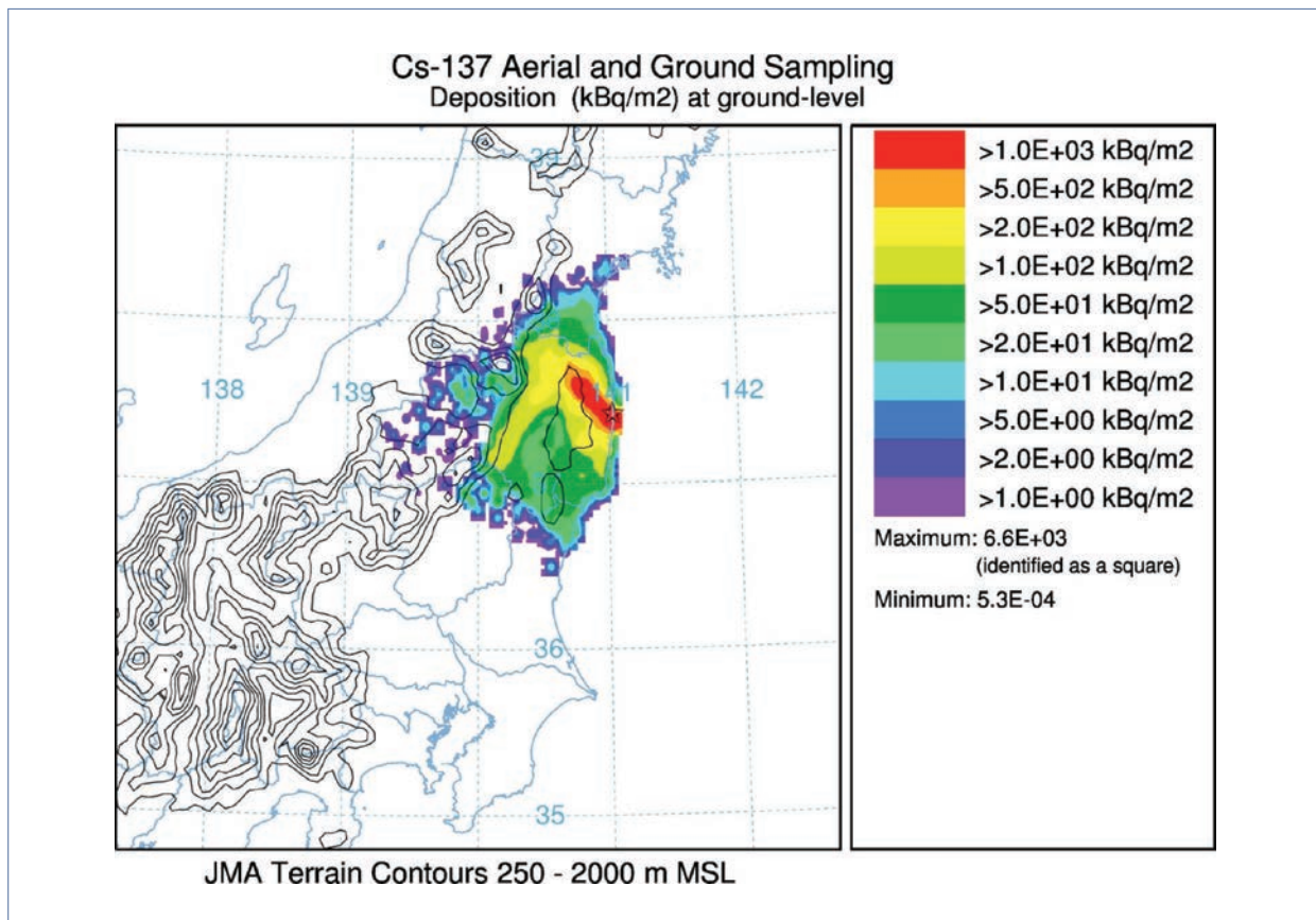
Figure 5. Measured Cs-137 deposition from ground (MEXT) and aerial (USDOE) sampling interpolated to the ATDM computational grid. Contours show the terrain elevation at 250 m intervals.
