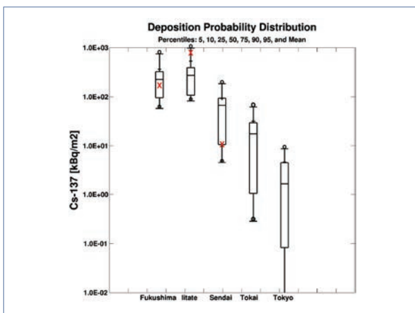
Figure 17. Box and whisker plot of the selected ensemble members for the total Cs-137 deposition at several locations. The red X shows the measured value at the grid cell corresponding to that location.
