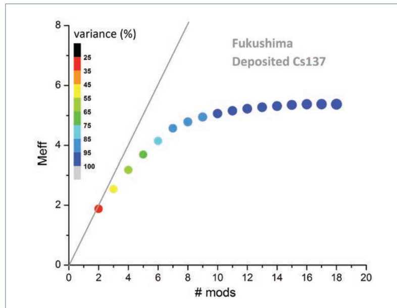
Figure 13. Variation of the effective number of members as a function of the ensemble size. The colours represent the variance of the ensemble.
