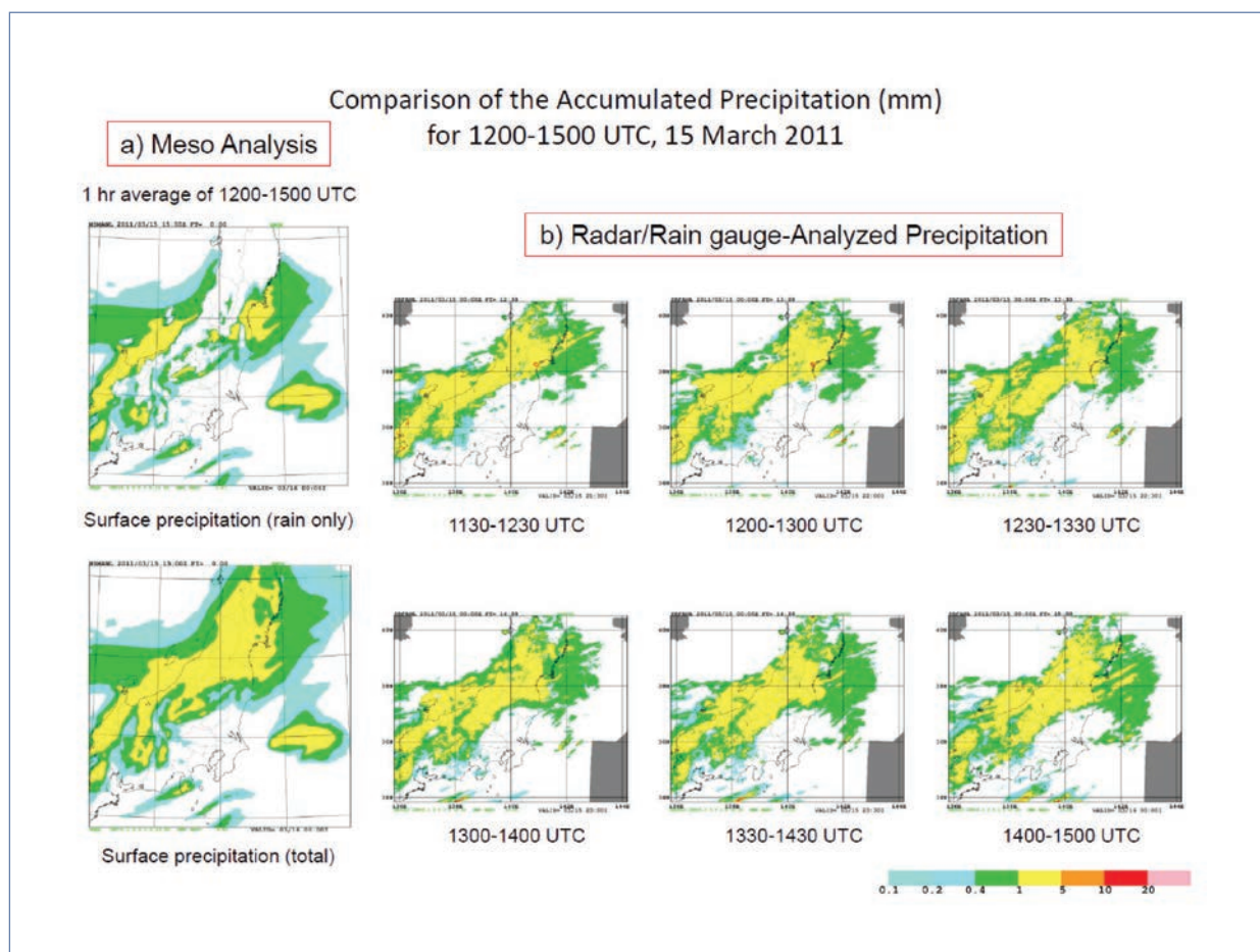
Figure 2. An example of the accumulated precipitation (mm) fields from (a) the JMA-MESO model analyses, and (b) the measured precipitation estimated from radar and rain gauge observations (RAP).
