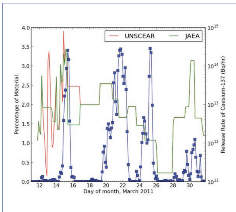
Figure 1. Time evolution of the percentage of modeled UKMET – ECMWF (blue line) total deposition (throughout March) in the region where measurements are available by each three hour source, assuming that the release rate of all sources was 1Bq/hr compared to emission rates of Cs-137 for the UNSCEAR and JAEA source terms.
