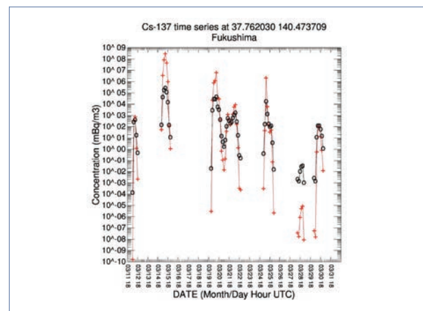
Figure 18. The calculated Cs-137 air concentration time series at Fukushima City (black o) and the ensemble variance for each calculation (red +). Variance units are concentration squared.
