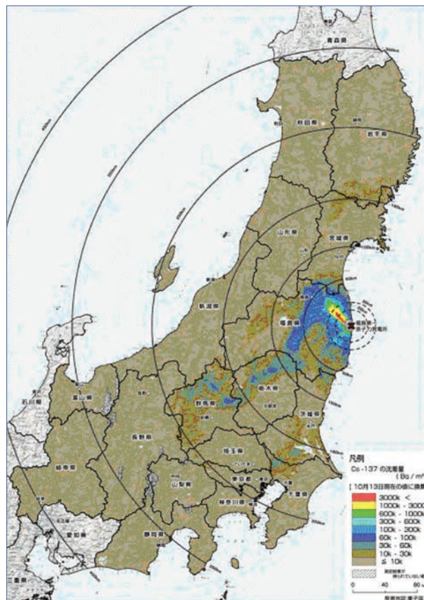
Figure 4. Regional deposition map of Cs-137 from MEXT (2011).
