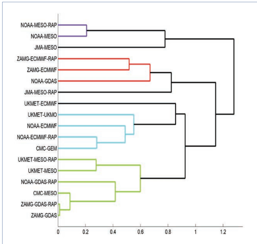
Figure 15. Dendrogram of the ensemble
