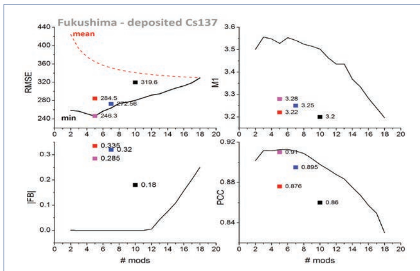
Figure 16. Performance of alternative sets (see the text for a description of the colours) compared with the minimum set and the minimum performance per number of members.
