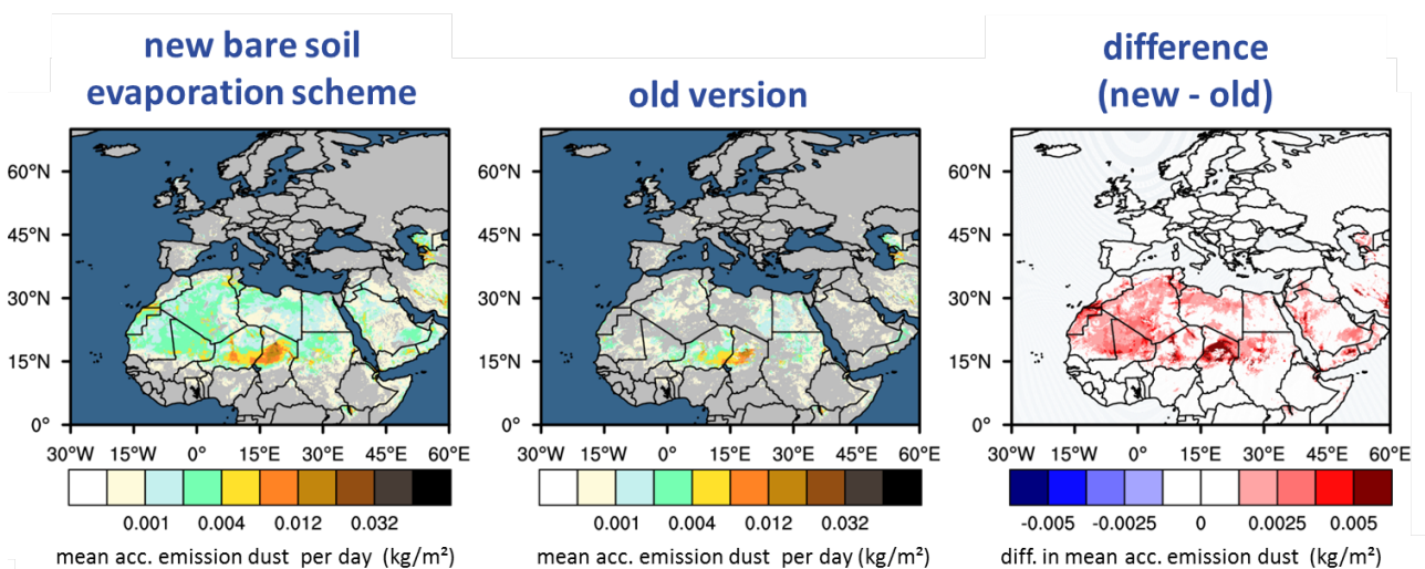
Figure 3: Mean accumulated mineral dust emission (10 February 2017 – 15 March 2017) using the new (left) and the old (middle) bare soil evaporation scheme as well as their difference (right).
