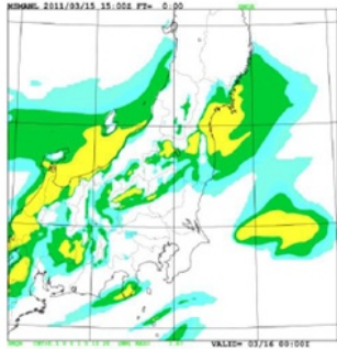
Surface precipitation (rain only)
