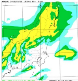
Surface precipitation (total)
