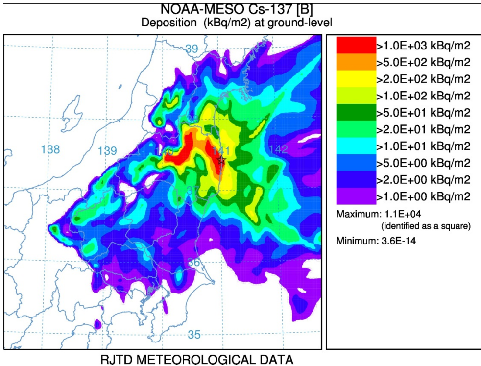
Figure 6. Calculated Cs-137 deposition using NOAA-HYSPLIT ATDM with ECMWF data (A - top) and with the JMA-MESO analysis (B - bottom).
