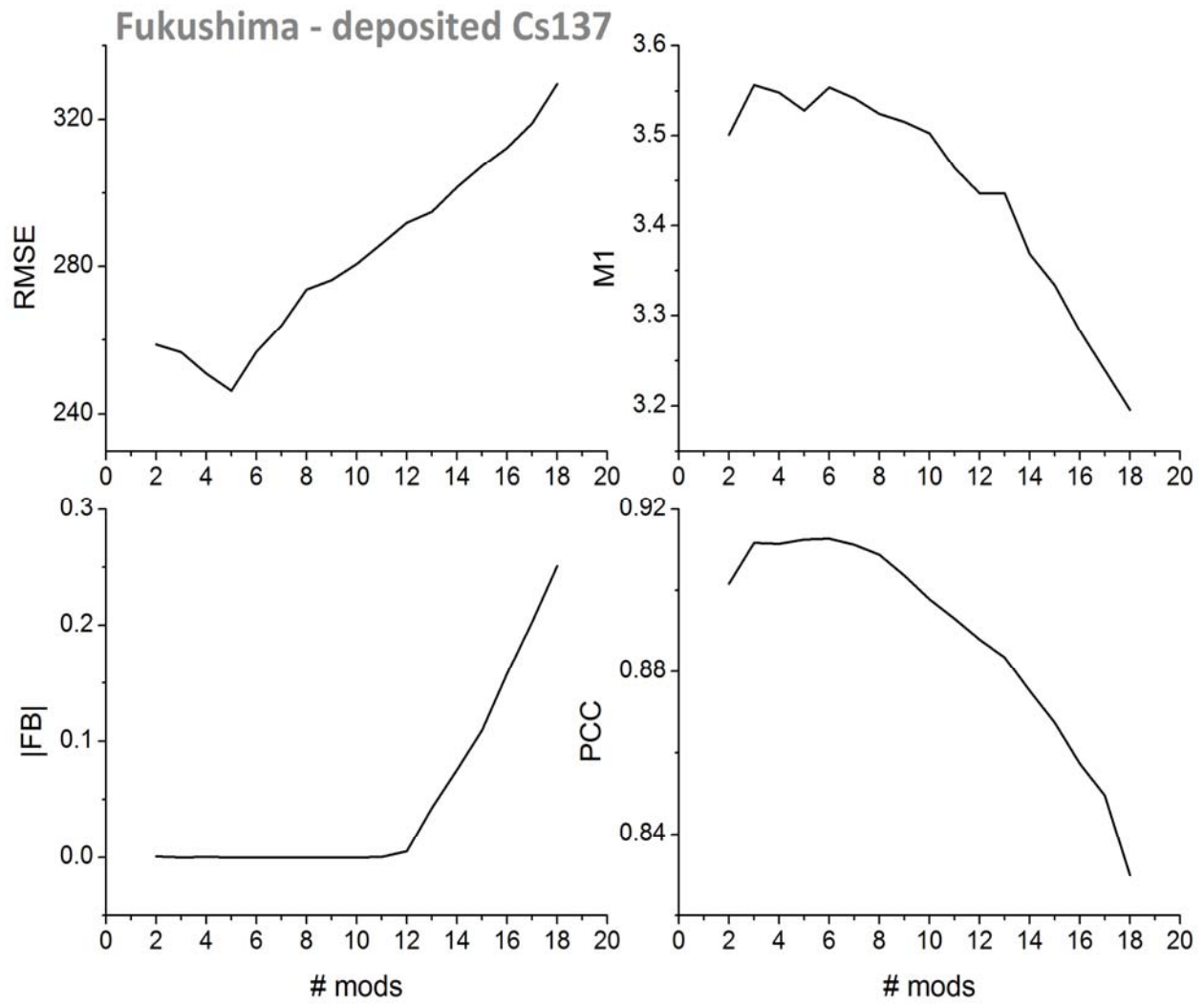
Figure 14. Clockwise from top left curves of minimum RMSE, maximum M1, maximum PCC, minimum FB, as a function of the number of models.
