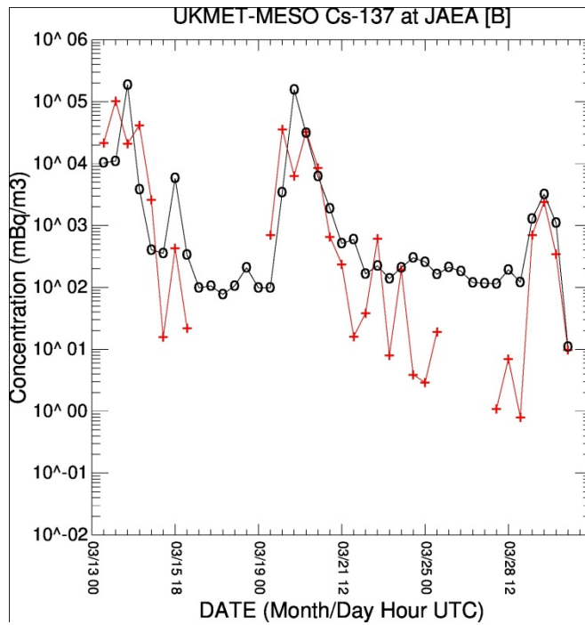
Figure 11. Calculated Cs-137 air concentrations (red +) using UKMET-NAME ATDM with ECMWF data (A - top), JMA-MESO analysis (B - bottom), and the measured data at JAEA (black o).
