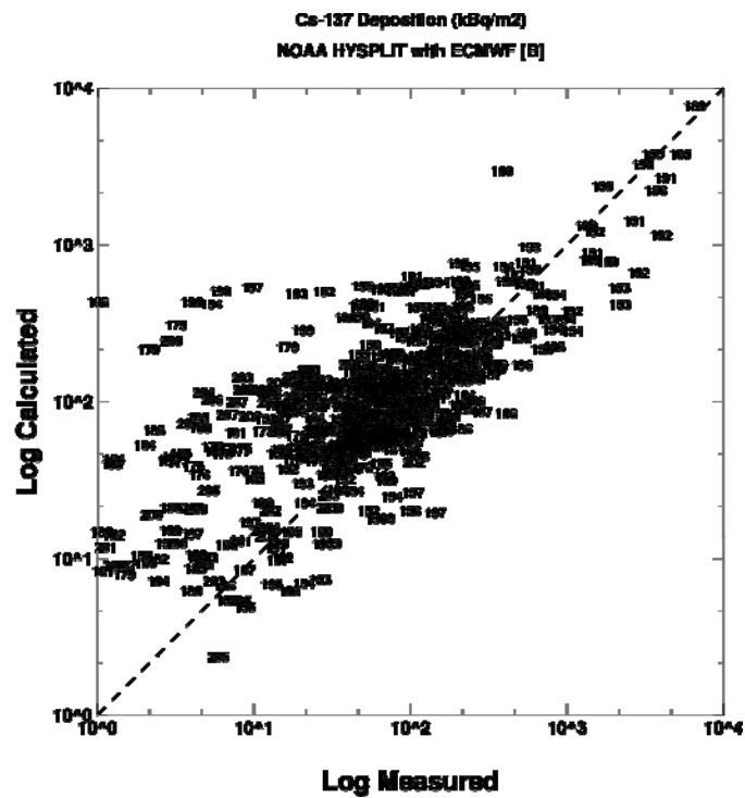
Figure 9. Scatter diagram for Cs-137 deposition for the ensemble mean model (A - top) and the NOAA-HYSPLIT using the ECMWF data, the model with the highest rank (B – bottom). Numbers represent the grid cell position in sequential units.
