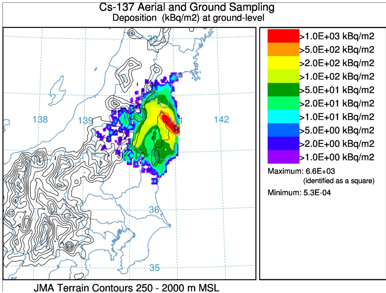
Figure 5. Measured Cs-137 deposition from ground (MEXT) and aerial (USDOE) sampling interpolated to the ATDM computational grid. Contours show the terrain elevation at 250 m intervals.
