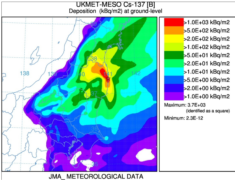
Figure 7. Calculated Cs-137 deposition using UKMET-NAME ATDM with ECMWF data (A - top) and with the JMA-MESO analysis (B - bottom).
