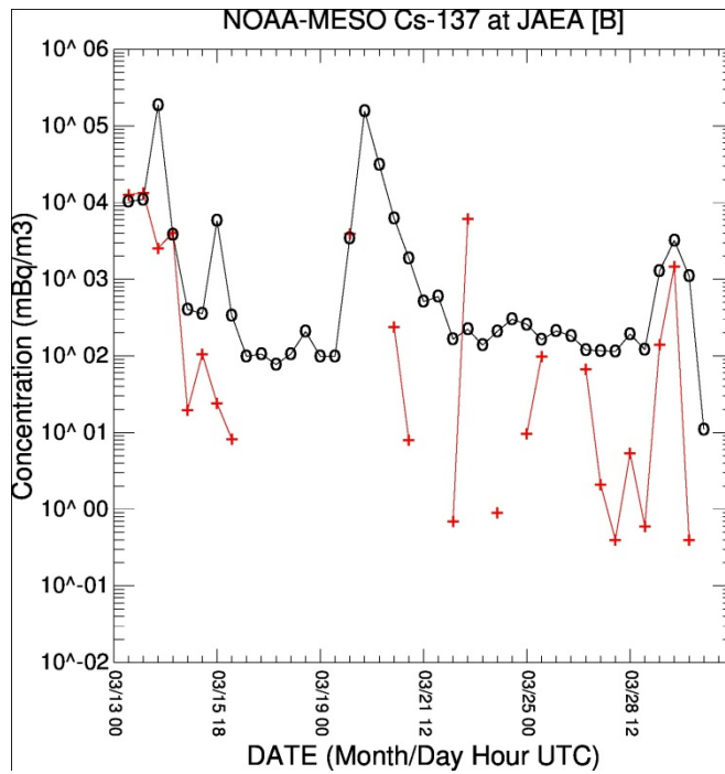
Figure 10. Calculated Cs-137 air concentrations (red +) at JAEA using NOAA-HYSPLIT ATDM with ECMWF data (A - top), with the JMA-MESO analysis (B - bottom), and the measured data at JAEA (black o).
