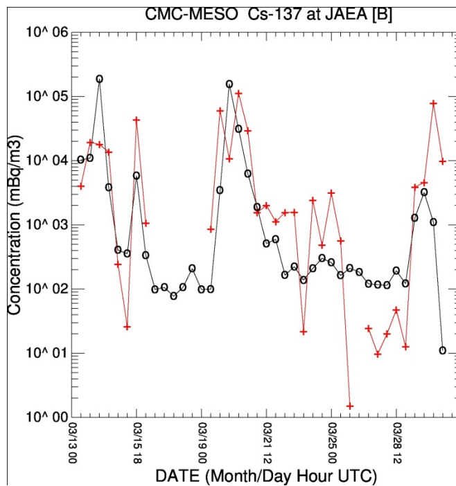
Figure 12. Calculated Cs-137 air concentrations (red +) using the ENS-Mean ATDM (A - top), CMC-MLDP0 using JMA-MESO (B - bottom), and measured data at JAEA (black o).
