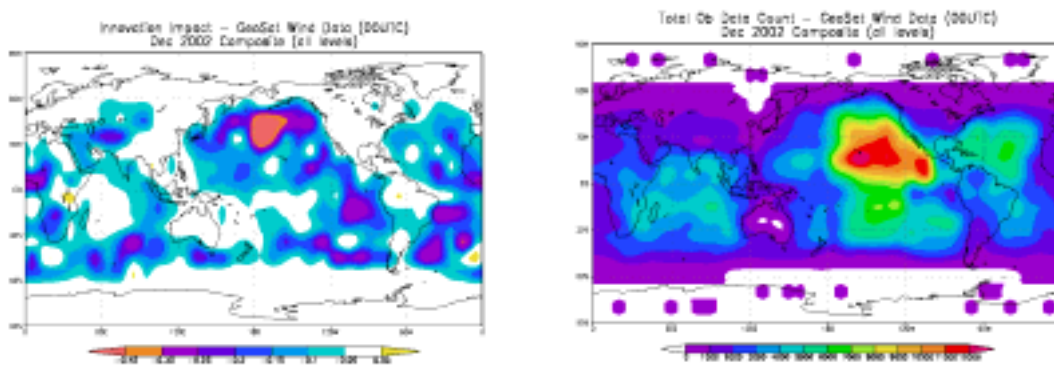
Figure 4.2: Left panel, estimated cumulative impact of all geostationary satellite wind observations (at 00UTC) on reducing December 2002 24-hr global forecast errors. Negative values indicate a reduction in forecast errors of combined temperature, wind, pressure (all levels, units = J kg -1 ) due to assimilation of the wind observations. This calculation involves the adjoint versions of the NAVDAS 3d-Var assimilation procedure and NOGAPS forecast model. Right panel, total number of satellite wind observations during the same period. Figure courtesy of Rolf Langland (Naval Research Laboratory, Monterey, CA).
