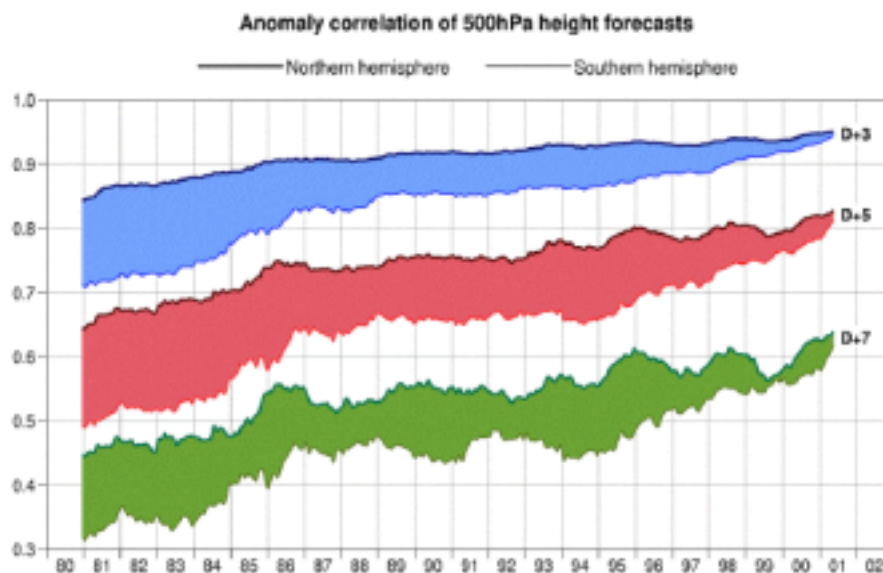
Fig.1.1: Evolution of forecast skill for the northern and southern hemispheres: 1980-2001. Anomaly correlation coefficients of 3, 5, and 7-day ECMWF 500-mb height forecasts for the extratropical northern and southern hemispheres, plotted in the form of running means for the period of January 1980-august 2001. Shading shows differences in scores between hemispheres at the forecast ranges indicated (from Hollingsworth, et al. 2002).
