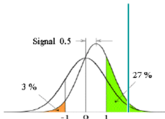
Fig 2.2: Schematic probability density functions illustrating the climatology (with zero mean), and the forecast PDF (displaced from zero mean) at some forecast lead time evolved from an initially narrow PDF (blue vertical line). For the EPS to be reliable, the verifying analysis at that lead time must fall within the climatology. The coloured areas indicate the chances of the verifying analysis falling at the extremes of the climatology, which are substantially different from the 16% chance expected from climatology.
