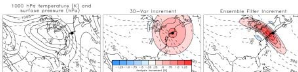
Figure 4.3: Illustration of the impact of background-error covariances. The surface pressure and 1000 hPa temperature of the model first guess are shown in the left-hand panel. Consider the correction, or “increment,” to an observation that is 1K warmer than the first guess at the location denoted with a dot. 3D-Var increments (middle panel) are isotropic, largest at the observation location and smaller with increasing distance from the observation. Ensemble-filter increments use flow-dependent background-error covariances that recognize that errors are more strongly correlated along the warm front than across it; hence corrections are stretched out along the frontal zone and maximized not at the observation location, but nearby where the gradient is tightest. Figure courtesy of Tom Hamill.
