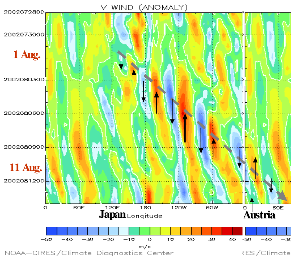
Fig. 2.1: Hovmöller (time-longitude) diagram of the 250-mb meridional wind component ( \text{ms}^{-1} ) for the period 28 July - 14 August 2002 and the latitudinal belt 40\text{--}60^\circ N. Extreme flooding in central Europe occurred at the end of this period. A Rossby wave train was excited by cyclogenesis off Japan, followed by rapid downstream development of high-amplitude Rossby waves, culminating in the severe weather in Europe. A skillful forecast of the cyclogenesis east of Japan is necessary to obtain skillful medium-range forecasts over Europe.
