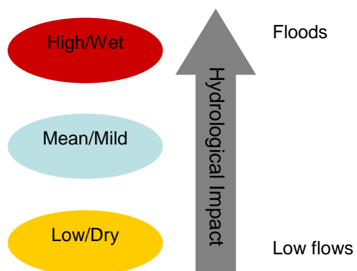
Figure 5. The three climate scenarios for Belgium: high/wet, mean/mild and low/dry, representing pessimistic, mild and optimistic scenarios for flood and low flow studies, based on an ensemble of about 30 RCM runs and more than 20 GCM runs.
