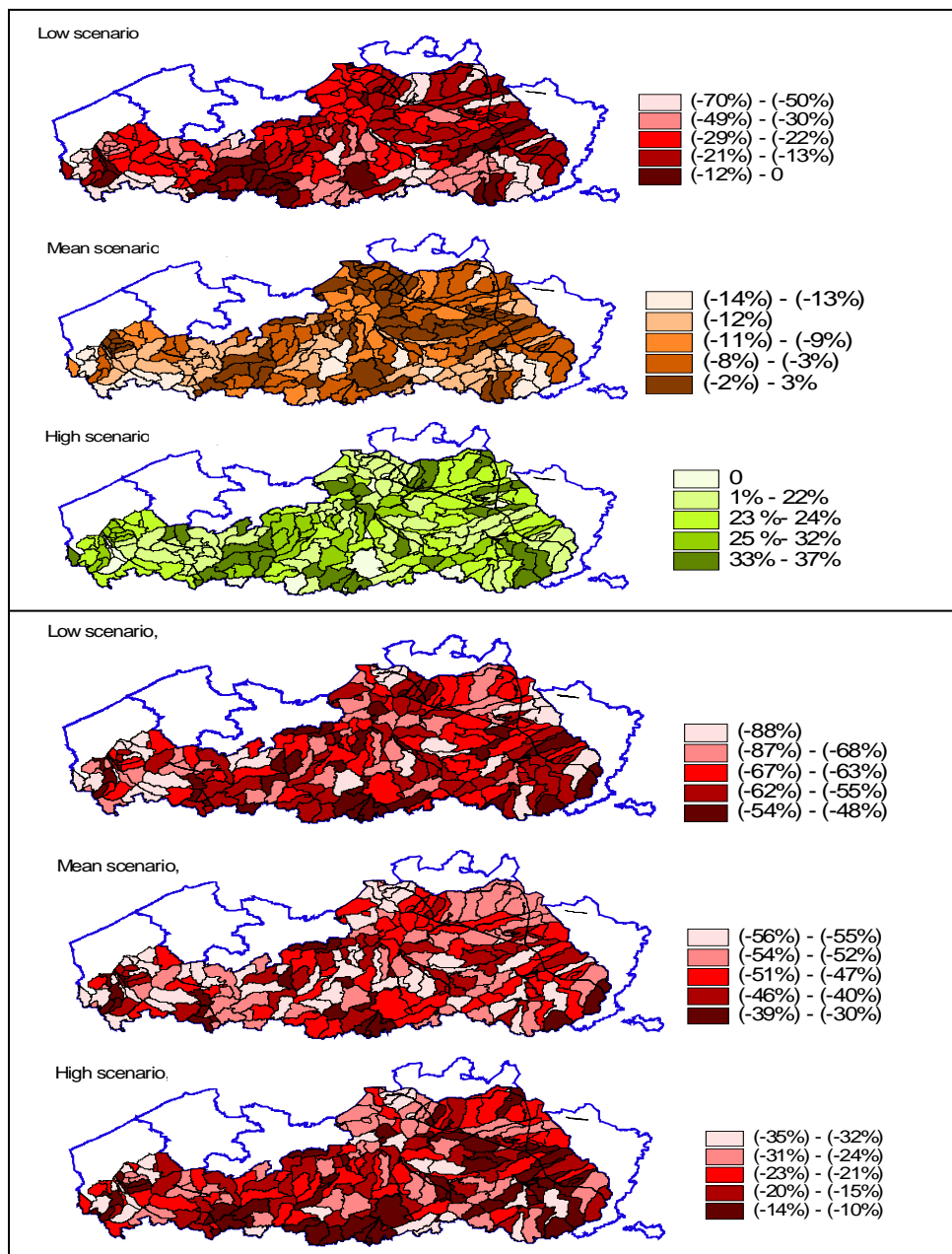
Figure 6. Percentage of variation (for the future climate 2071-2100 compared to the control period 1961-1990) of hourly runoff peaks (top panel) and low flows (down panel) for the low, mean and high climate scenarios and based on NAM lumped conceptual rainfall-runoff models.
