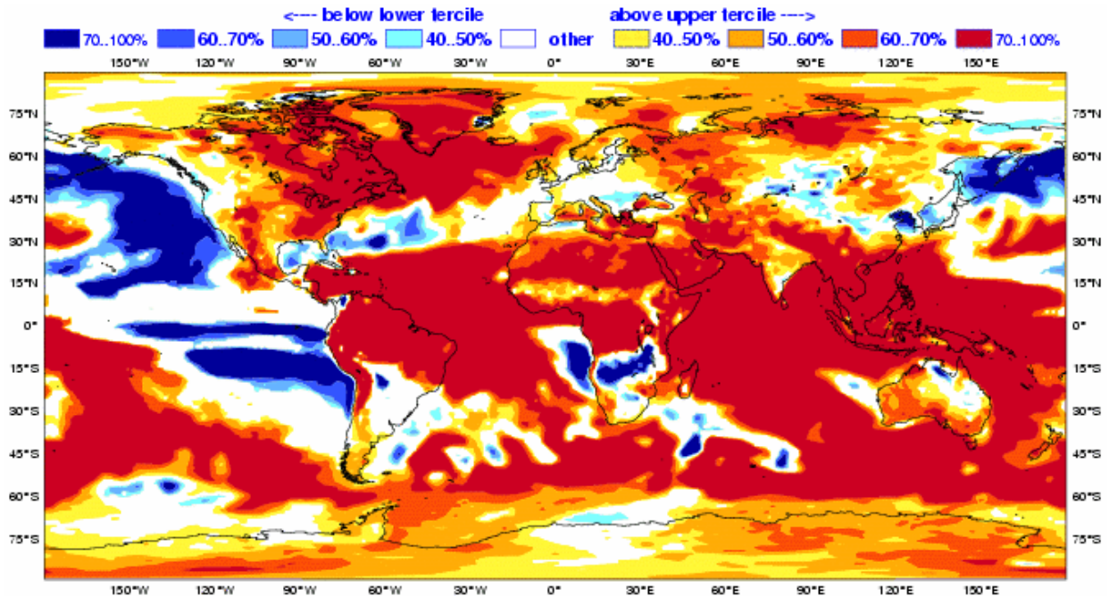
fig.10: Probabilistic forecasts for T2m from ECMWF for may-june-july, issued in April 2010. Most likely Category. (2 categories, Below and Above normal – white zones correspond to “Other”) http://www.ecmwf.int/products/forecasts/d/charts/seasonal/forecast/seasonal_range_forecast/grouop/
