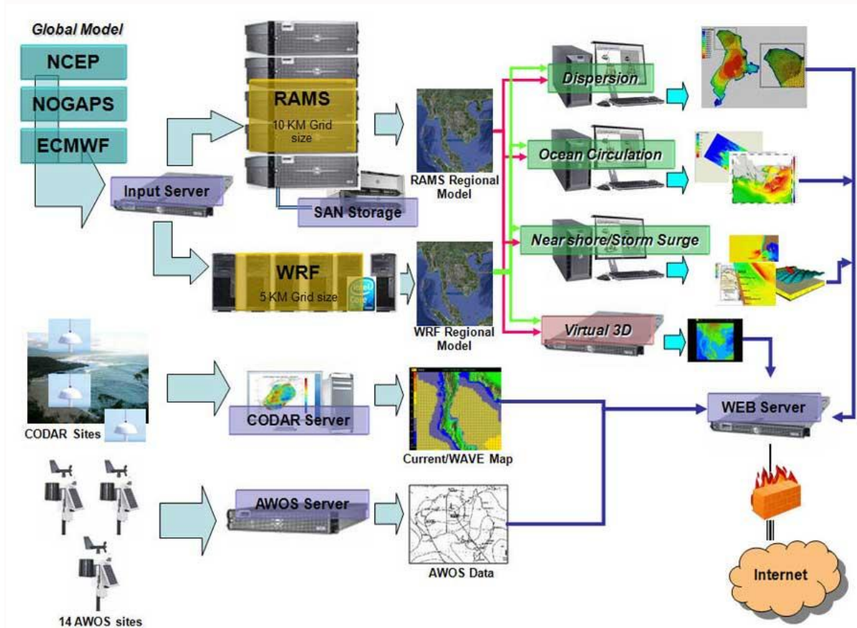
Marine Meteorological Disaster Warning System Flowchart.
