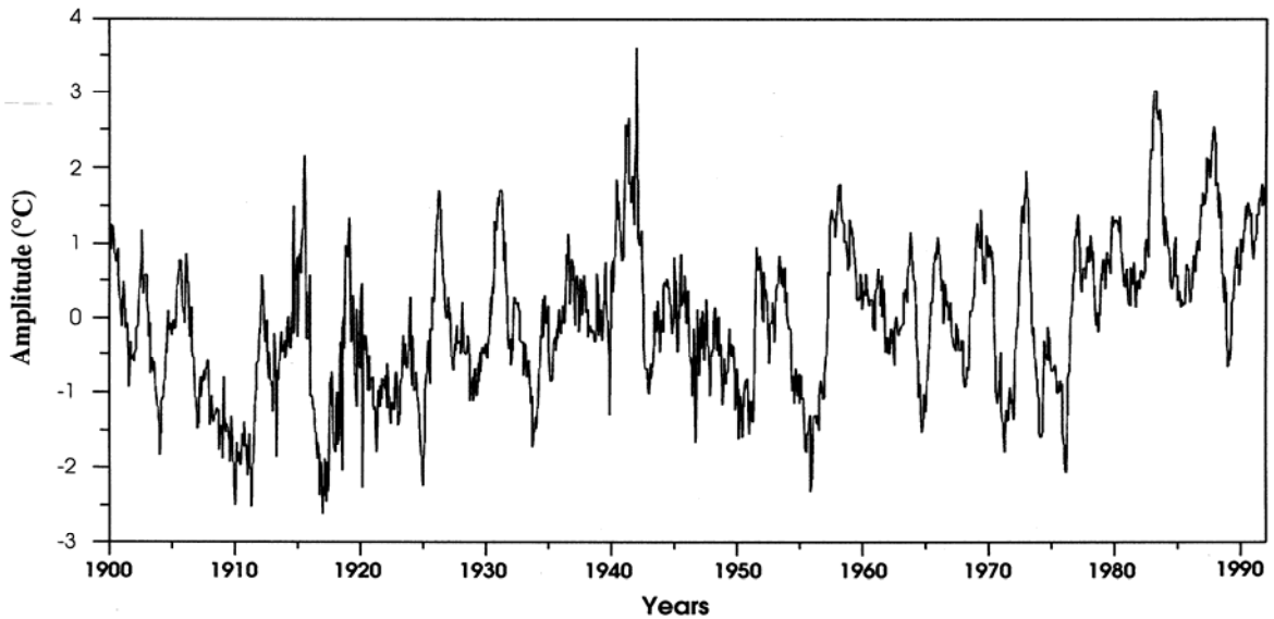
Figure 3: GOSTA global SST missing SVD analysis (rank=2). Estimated SST EOF2 amplitude.
