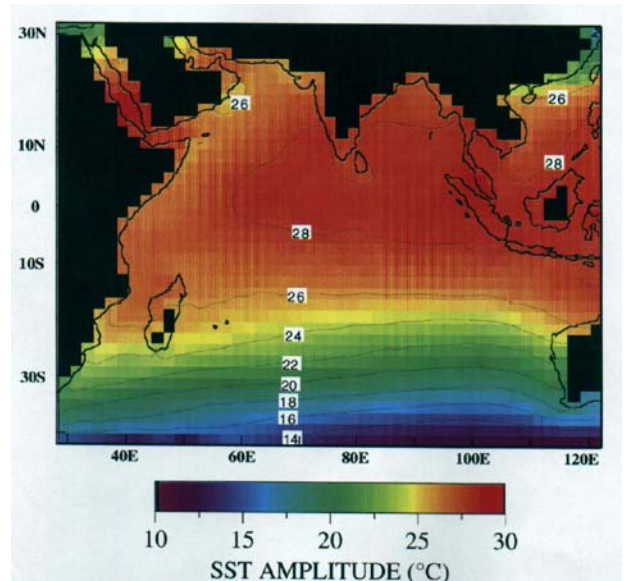
Figure 6: Indian Ocean SST estimated EOF1 (98.6%, rank=2).
