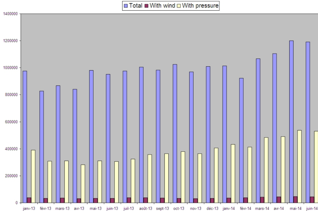
Time evolution of BUOY reports for wind and pressure
