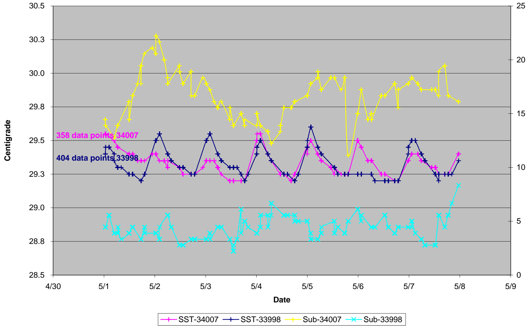
Comparison of 33998 (1.3 Watts) and 34007 (0.7 Watts)
