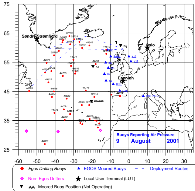
Figure 2. Distribution of EGOS buoys at August 9th, 2001.
