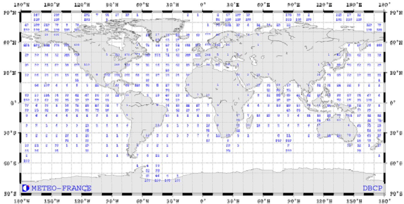
Figure 5. GTS data availability, April 2005 – Air temperature (by courtesy of Météo France).
