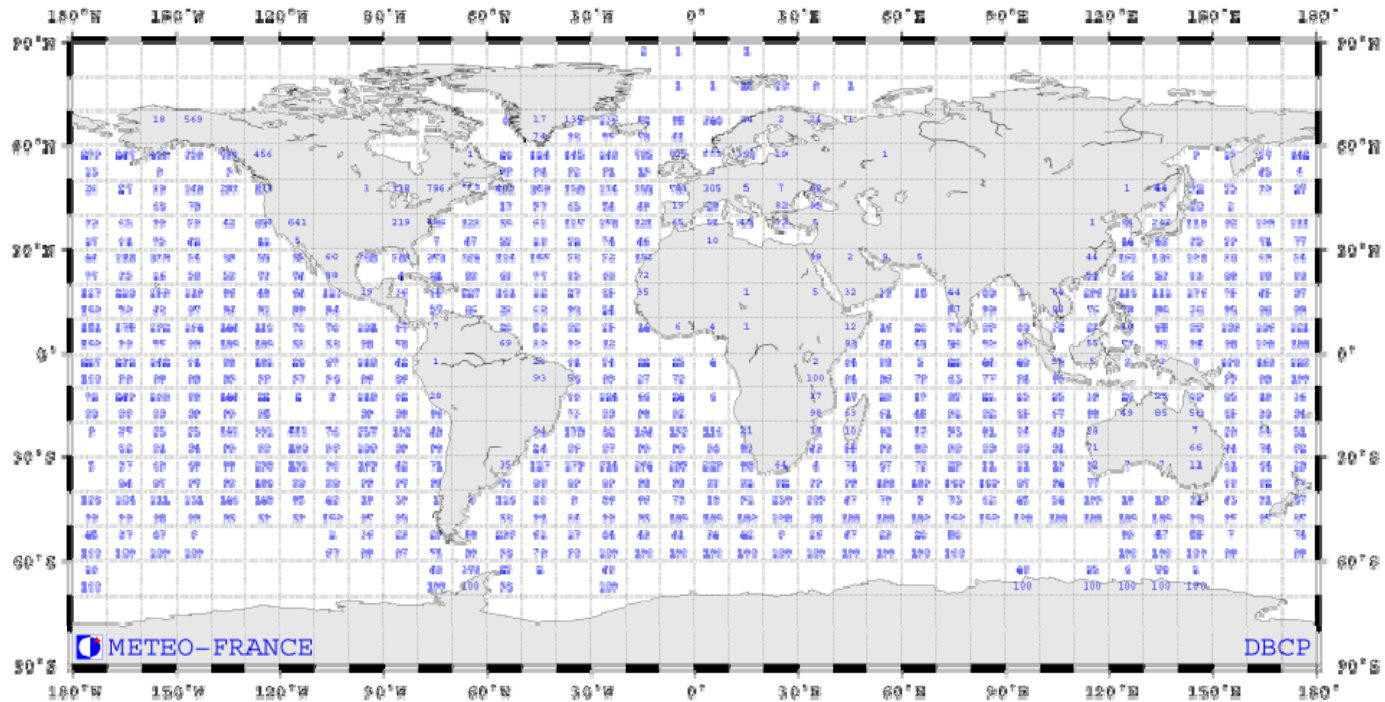
Figure 6. GTS data availability, April 2005 – Sea surface temperature (by courtesy of Météo France).
