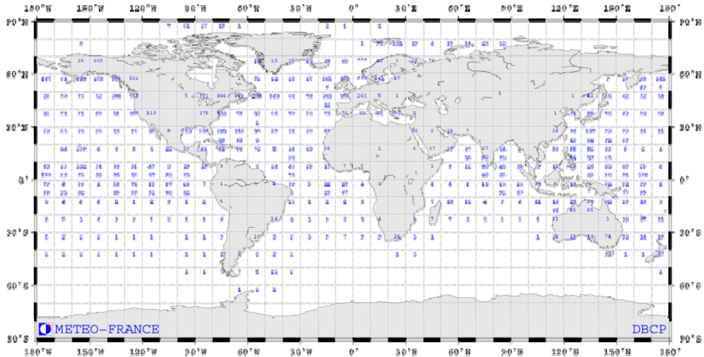
Figure 7. GTS data availability, April 2005 – surface wind (by courtesy of Météo France).
