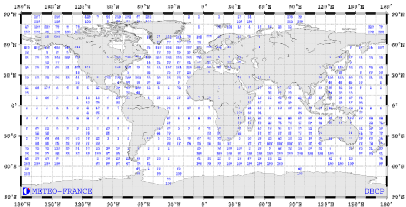
Figure 4. GTS data availability, April 2005 – Surface atmospheric pressure (by courtesy of Météo France).
