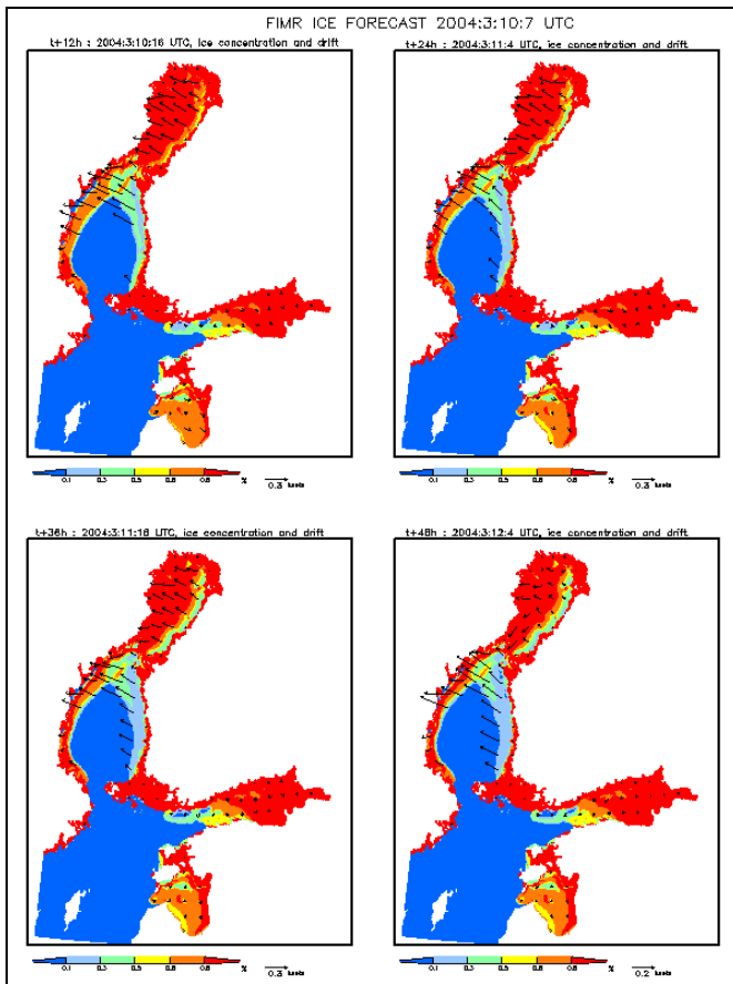
Figure V-2. Ice concentration and drift forecast for 10-13.03.2005 (t+12h, +24h, +36h & 48h).
