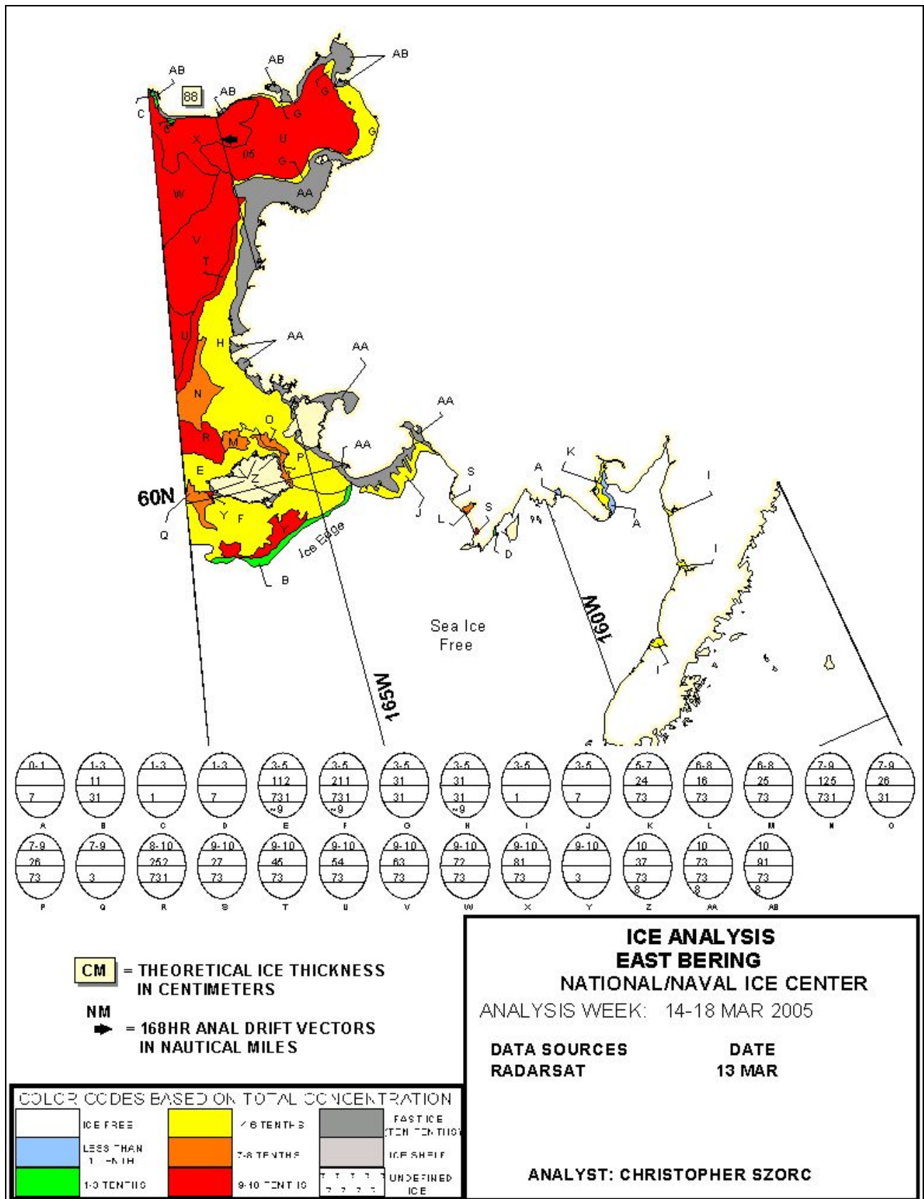
Figure XII-4 – Ice chart for the Eastern Bering Sea for 14 – 18 March 2005.
