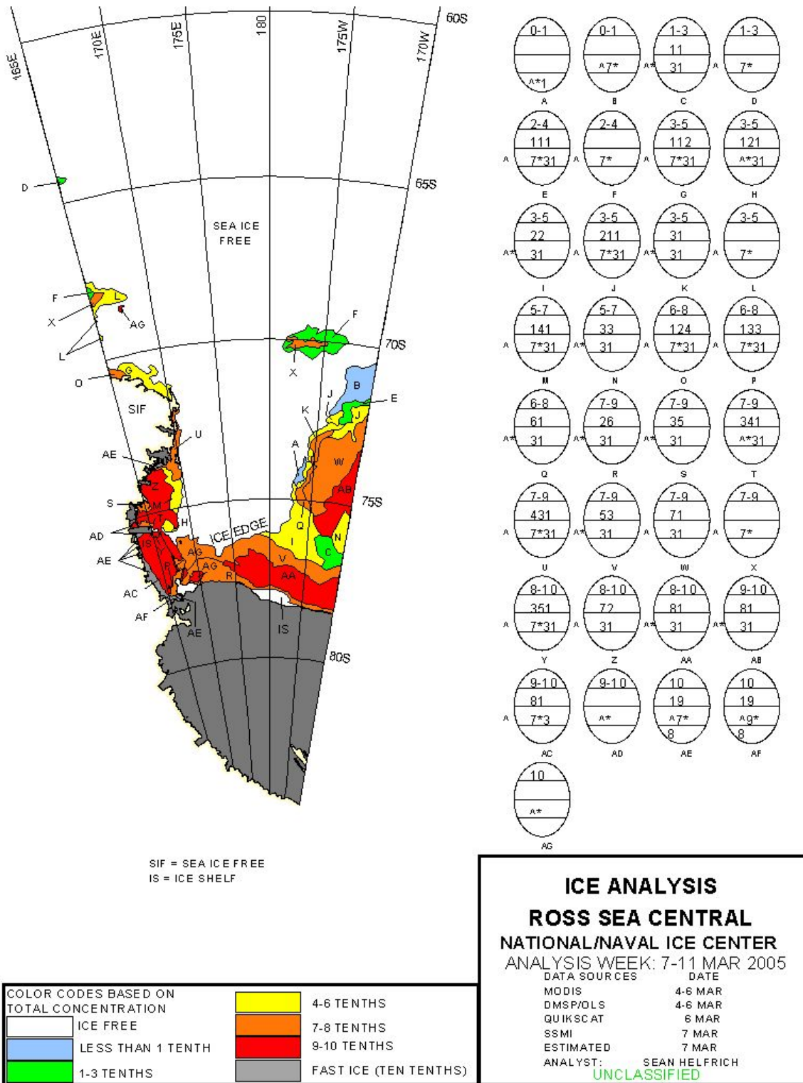
Figure XII-7 – Ice chart for the Central Ross Sea for 7 – 11 March 2005.
