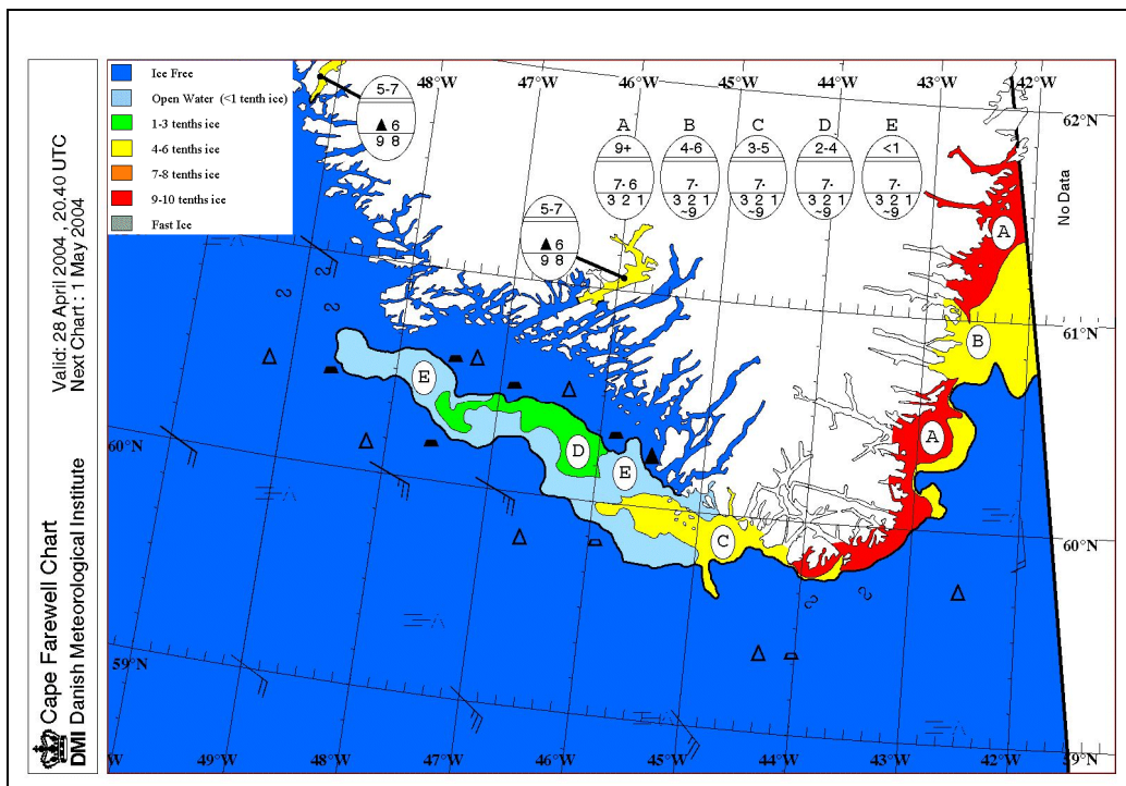
Figure III-4 – Cape Farewell ice chart for 28 April 2004.
