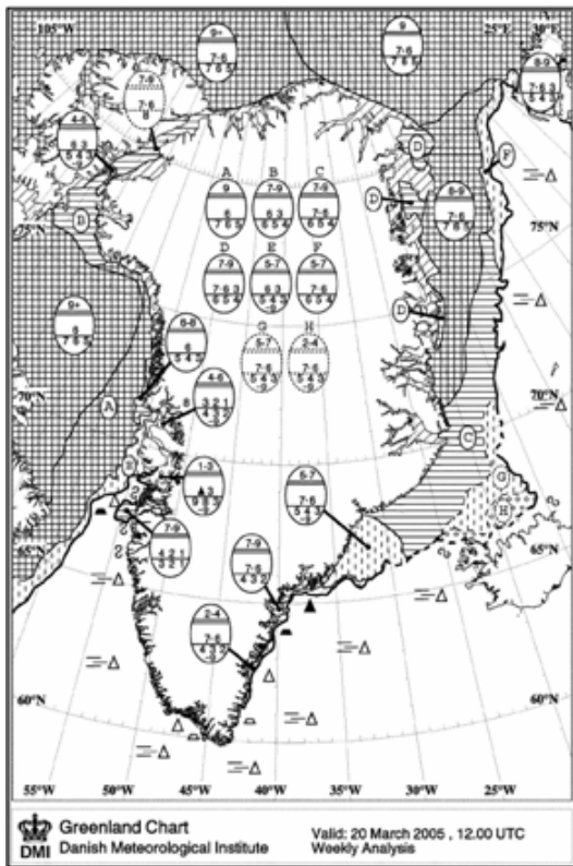
Figure III-2 – Weekly ice analysis for Greenland waters, 20 March 2005
