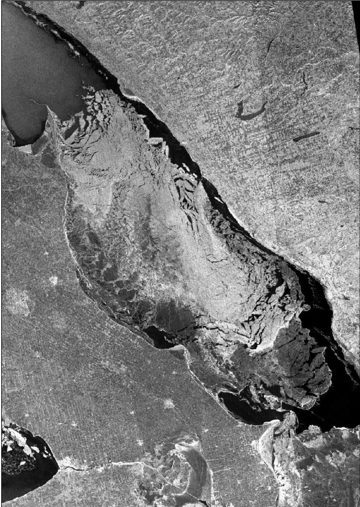
Figure I-7 – RADARSAT imagery for the Lake Erie
