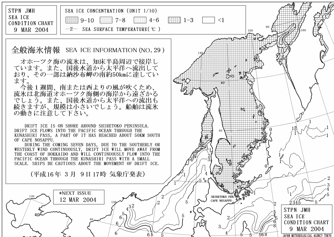
Figure VII-1 — Ice chart for the Sea of Japan and Sea of Okhotsk for 9 March 2004.
