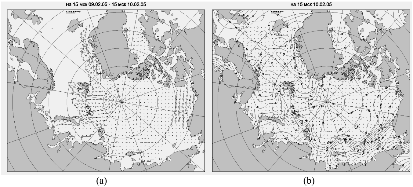
Figure X-3 – Forecast charts for the Arctic sea-ice drift (a) and currents and level elevation (b), 10 February 2005.
