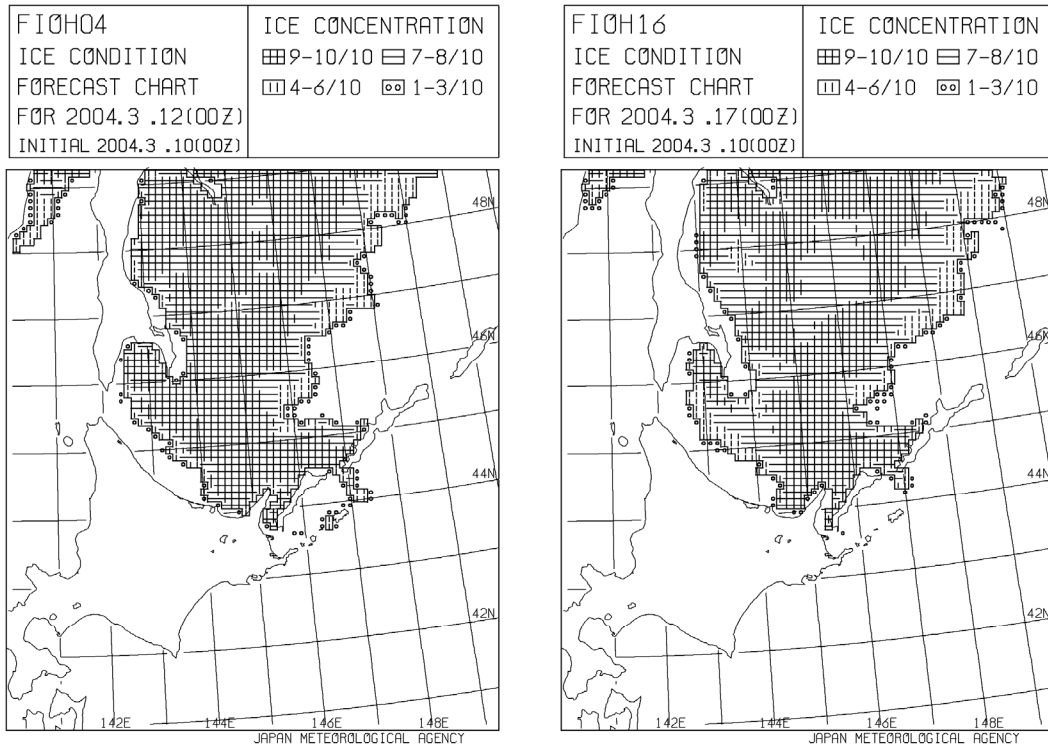
Figure VII-2 — Ice condition forecast charts for 12 and 17 March 2004 for the southern part of the Sea of Okhotsk(initial conditions from 10 March 2004).
