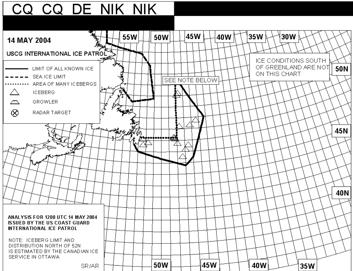
Figure XII-1 – Iceberg chart produced by the US Coast Guard International Ice Patrol for 14 May 2004.
