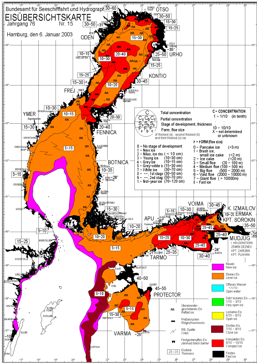
Figure VI-1. Ice chart for the Baltic proper northward of 56°N, 6 January 2003.
