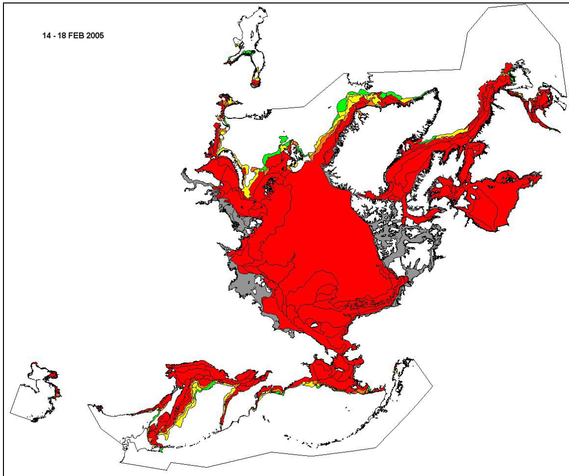
Fig.XII-8. Northern Hemisphere Sea Ice Analysis from ESRI ArcView for 14 – 18 February 2005.
