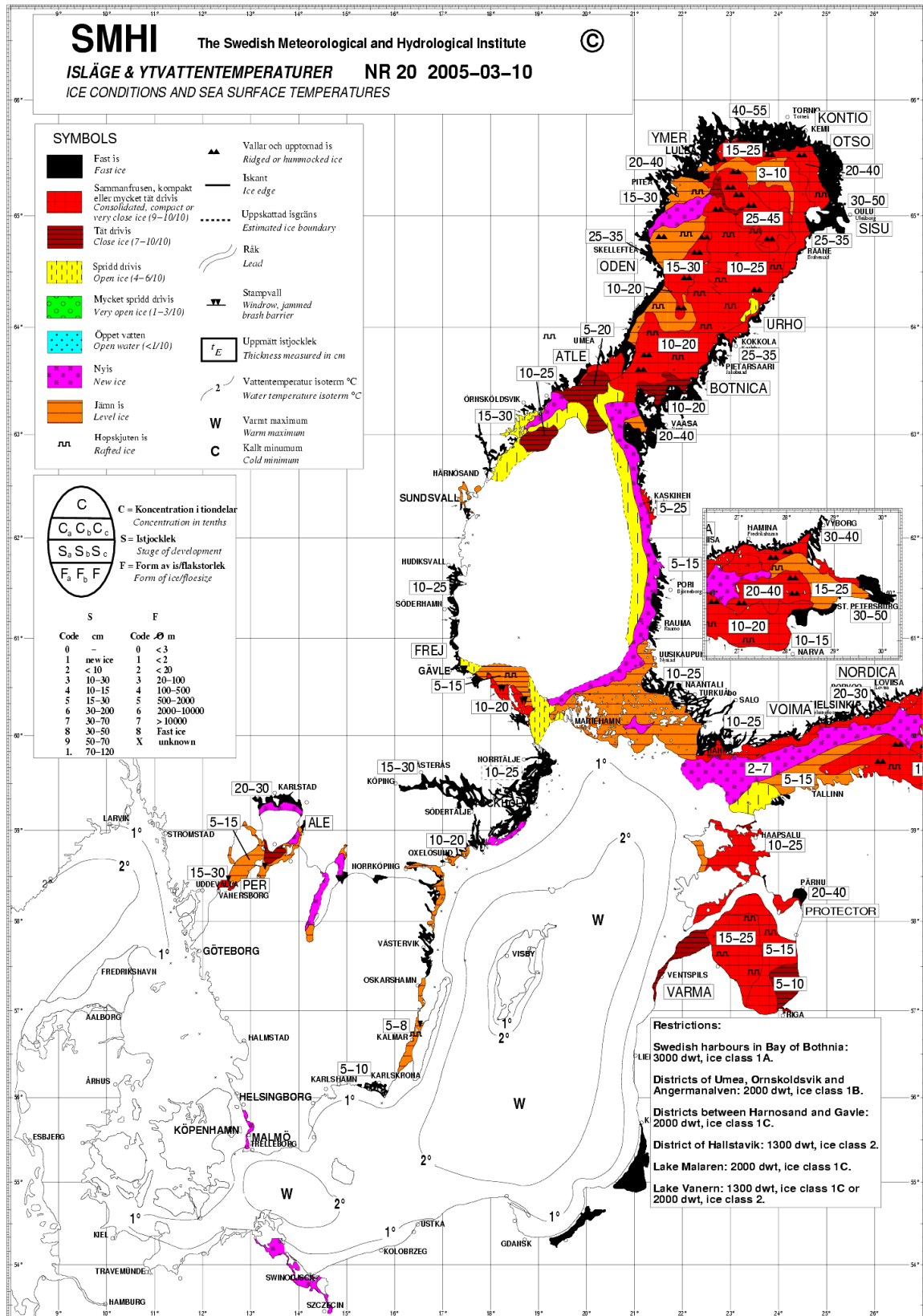
Figure XI-1 – Ice conditions and sea surface temperature chart for the Baltic Sea, 10 March 2005
