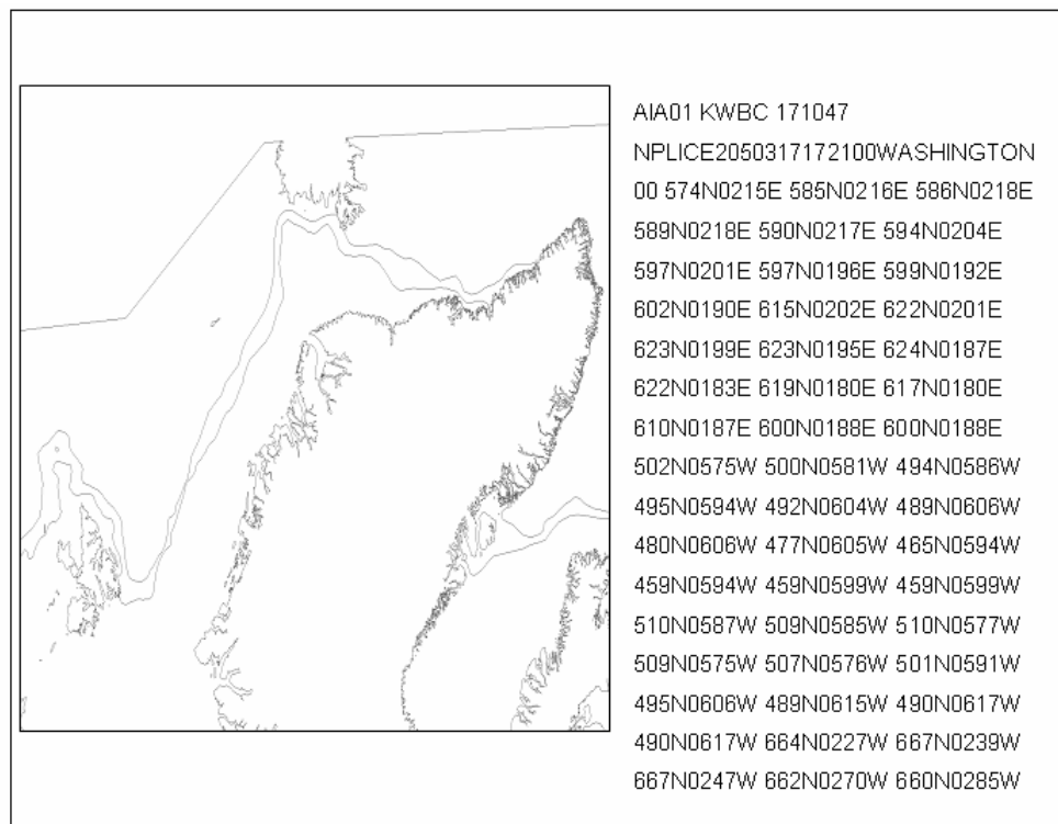
Figure XII-2 – Alphanumeric text message and corresponding graphical output for the ice edge position (Daily Ice Edge (DIE)) from 17 March 2005
