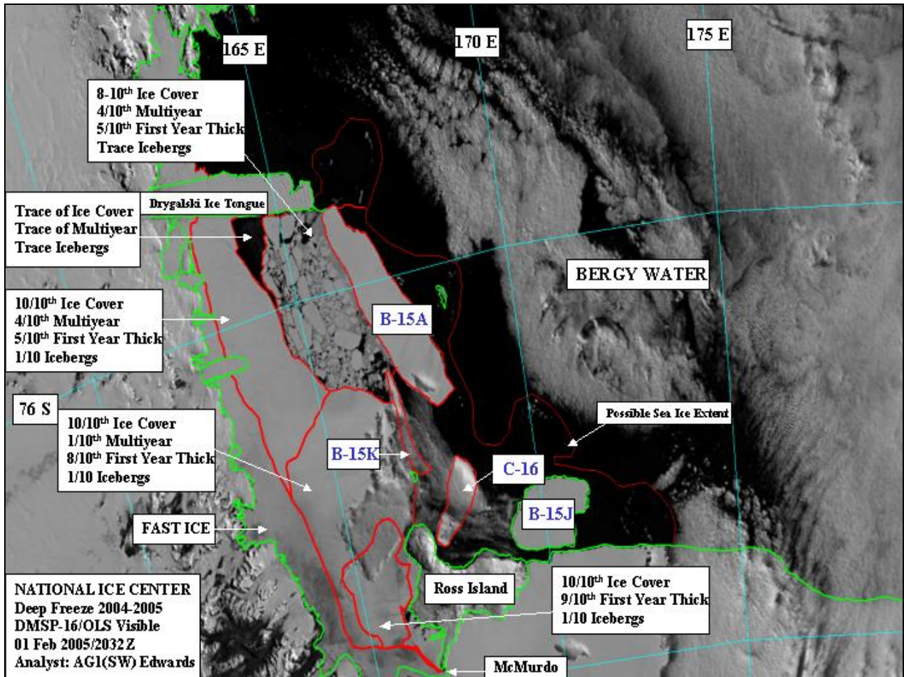
Figure XII-9 – Annotated special support product DMSP/OLS visible satellite image depicting tabular icebergs and sea ice in the Ross Sea on 01 February 2005 at 2032 UTC.
