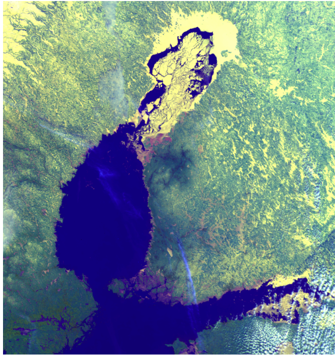
(a) Mosaic of NOAA AVHRR channels 1, 2 & 4 for 1 April, 2004. Captured and processed at SMHI.
