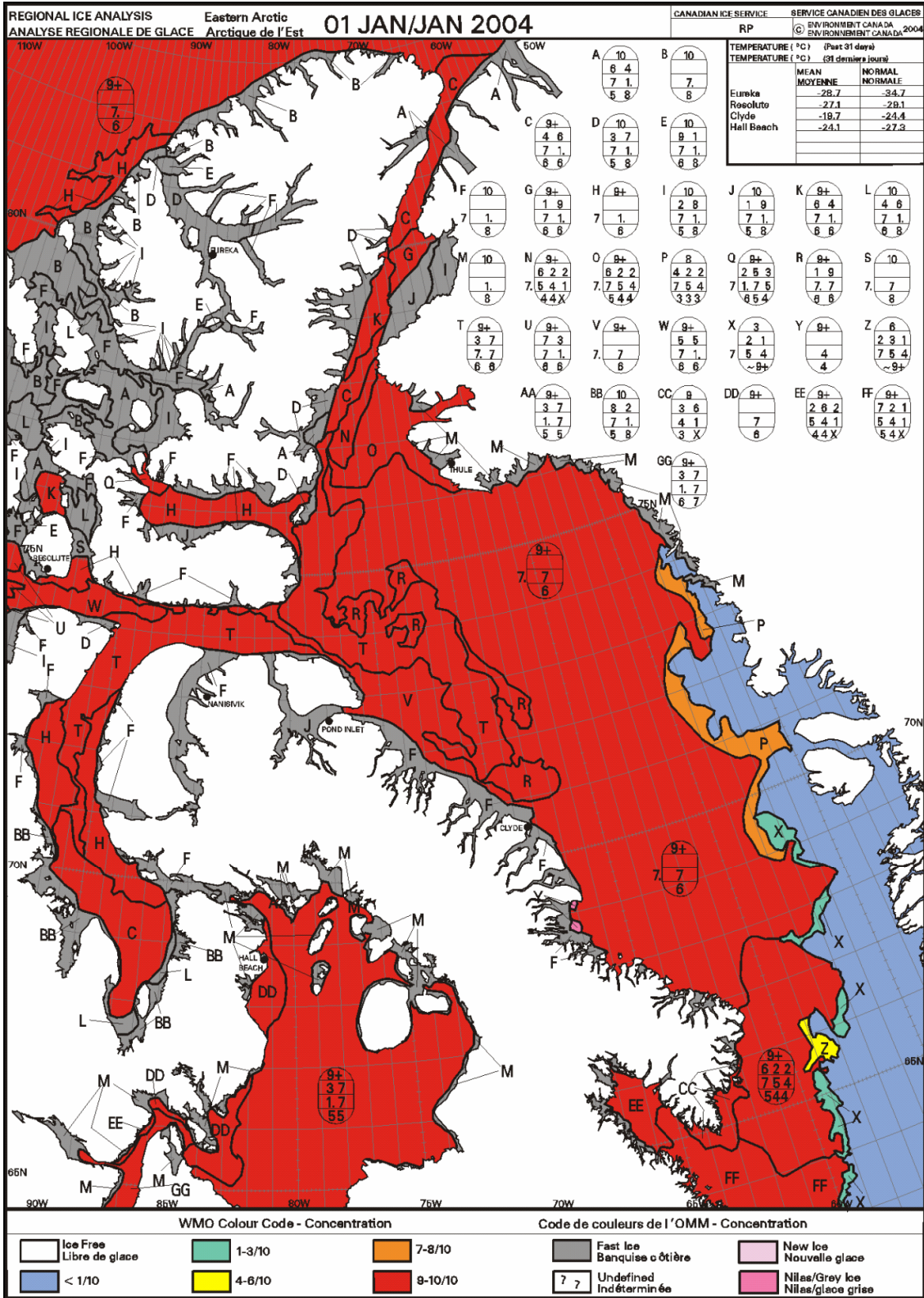
Figure I-1 – Regional weekly ice chart for the Eastern Canadian Arctic for 1 January 2004.
