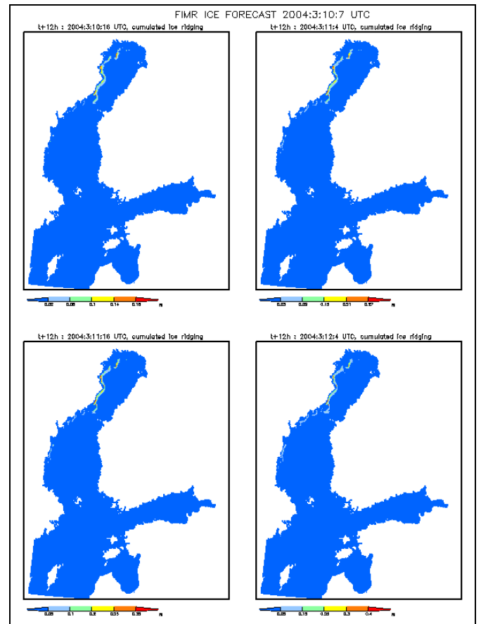
Figure V-3. Cumulated ice ridging forecast for 10-13.03.2005 (t+12h, +24h, +36h & 48h).
