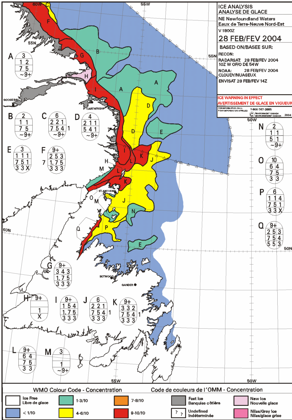
Figure I-3 – Daily analysis chart for Newfoundland
