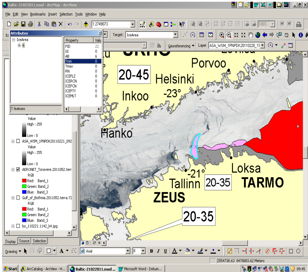
Figure 10 - Case Study 1b Detail of Ice Chart with Satellite Image Overlaid
