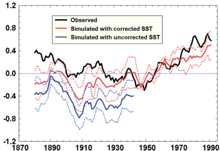
Figure 6. Approximately decadal filtered (21-point binomial filter) quasi-collocated observations (black curve) and HadAM3 ensemble mean anomalies from a 1946–65 average of annual mean LSAT for three corrected stations in southeast Australia, 1879–1990. Red (blue): with (without) bias corrections to SST. Light red and blue curves are \pm 2 standard errors of the ensemble means
