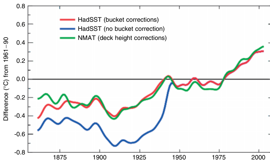
Figure 1. Influence of bias corrections on SST. The globally averaged HadSST1 data set with and without bias corrections (corrections cease at the end of 1941) is compared with bias-corrected global NMAT (HadMAT1). The data are approximately decadal averaged, using a 21-point binomial filter
