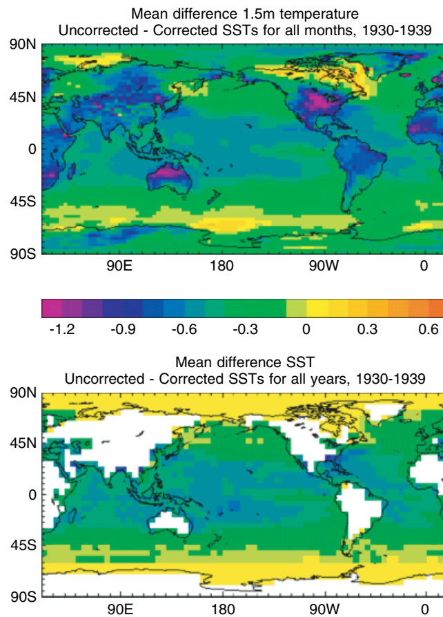
Figure 2. (a) Ensemble mean differences in 1.5 m simulated temperature for the decade 1930–39 between runs of HadAM3 forced with uncorrected GISST and bias-corrected GISST ( ^{\circ}\text{C} ). (b) Corresponding differences in imposed SST ( ^{\circ}\text{C} )
