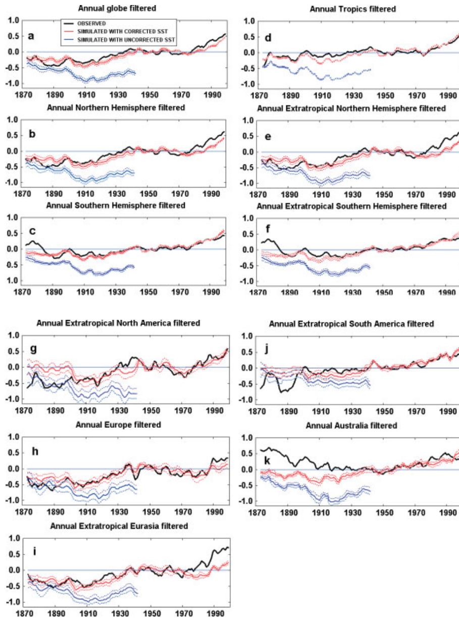
Figure 4. Near-decadally filtered (21-point binomial filter) collocated observations (black curve) and HadAM3 ensemble means of annual mean LSAT anomalies from a 1946–65 average for 11 regions, 1872–1998. Red (blue): with (without) bias corrections to SST. Red and blue dotted curves are \pm 2 standard errors of the ensemble means, calculated as in the text
