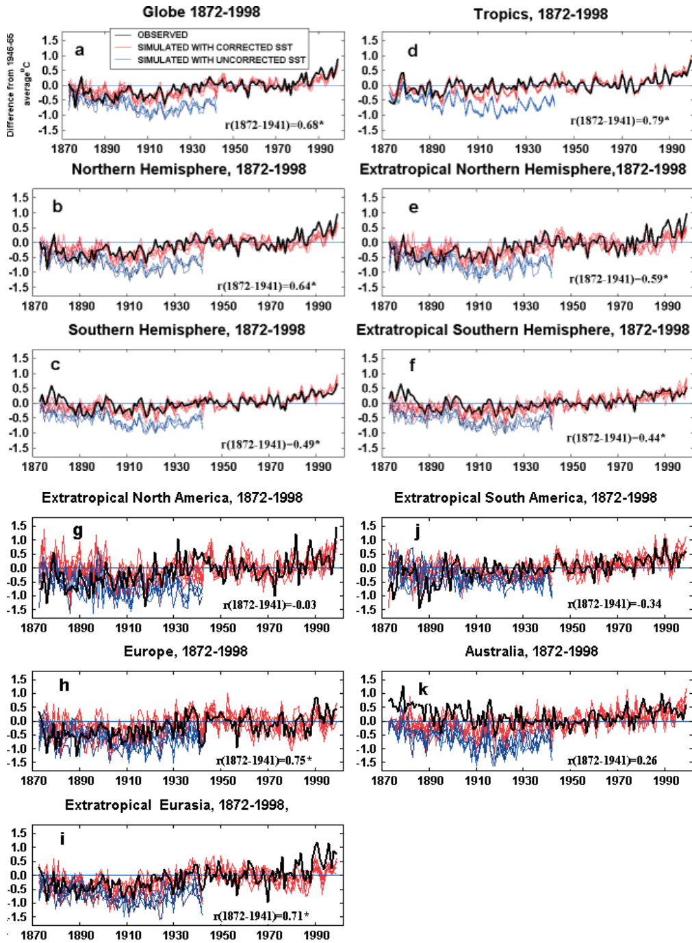
Figure 3. Unfiltered collocated simulations and observations (black curve) of annual mean LSAT anomalies from a 1946–65 average for 11 regions and for each HadAM3 ensemble member, 1872–1998. The six red curves in each plot derive from simulations with SST bias corrections up to 1941 inclusive, with no corrections thereafter. The four blue plots are derived from simulations without bias corrections up to 1941
