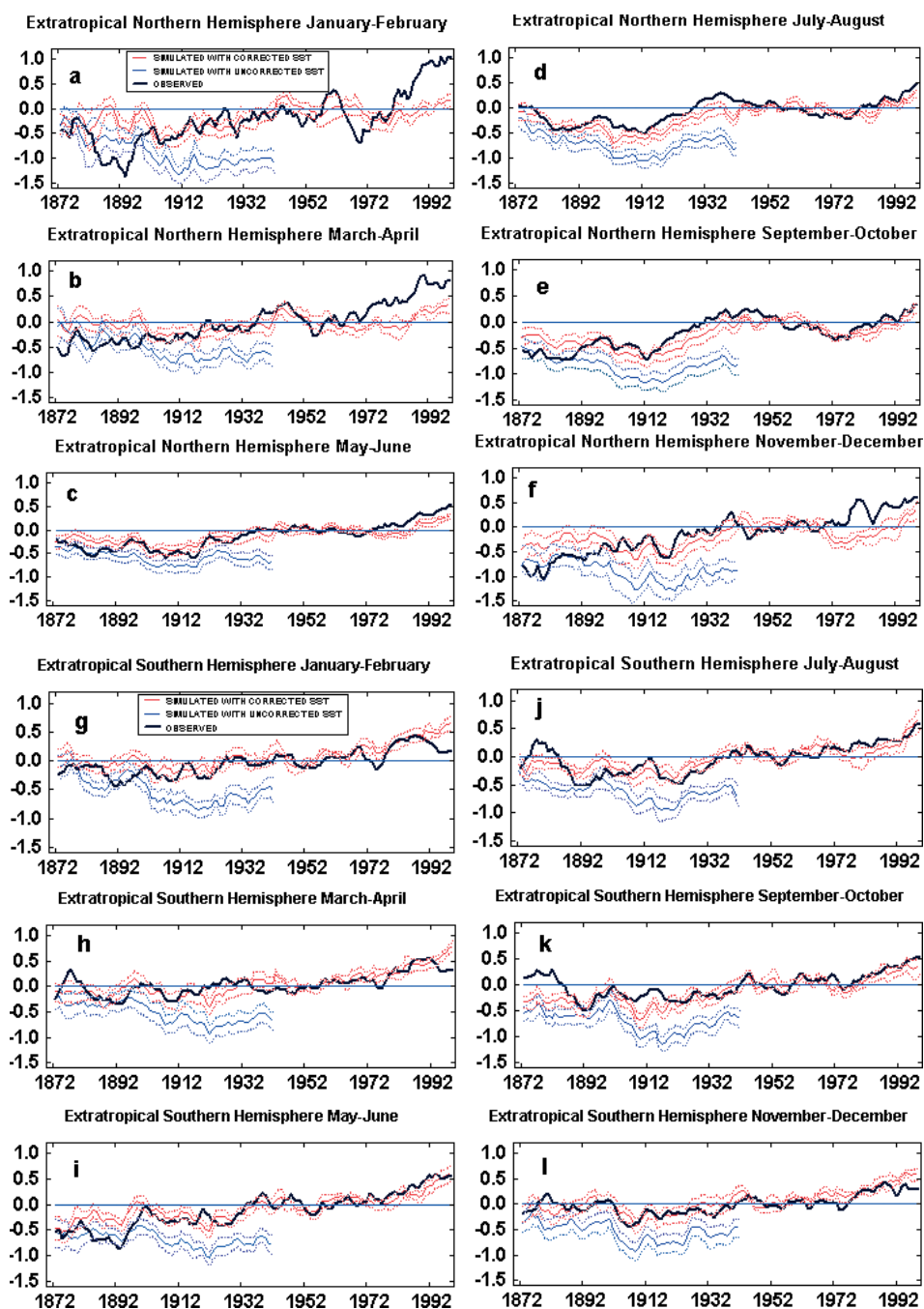
Figure 7. Simulations of seasonally varying approximately decadal averaged LSAT using SST with and without bias corrections for the extratropical Northern and Southern Hemispheres, 1872–1998, using the conventions of Figure 4. Two-month seasons January–February, March–April, etc. The observations are in black
