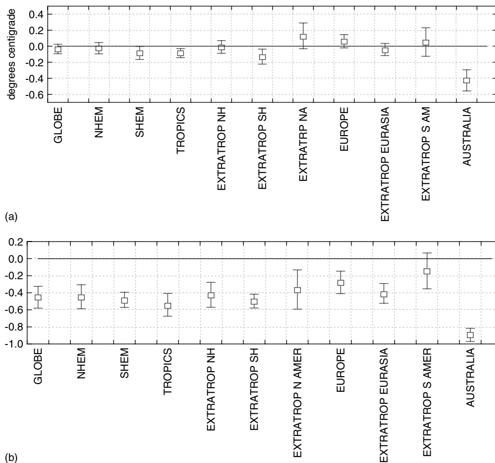
Figure 5. (a) Differences between bias-corrected simulations of annual mean LSAT anomalies from a 1946–65 average and observed (Jones et al. , 1999) annual mean LSAT anomalies from the same period over the whole period of bias corrections, 1872–1941. (b) As (a), but simulations using uncorrected SST data
