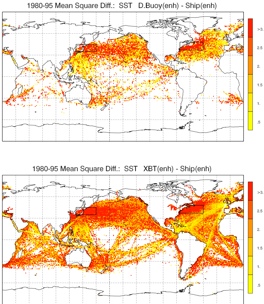
Fig.1 Spatial pattern of mean square differences between the SST measured by drifting buoys, XBT, and the SST observed by ships. The boxes in the northwest Pacific ocean and northwest Atlantic ocean indicate the areas for which spatial average of the buoy/ship and XBT/ship differences are shown in table 1.
