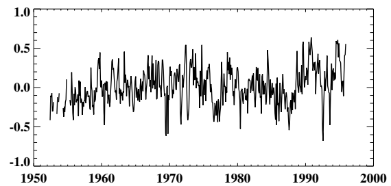
Fig.2b Upper panel: PC-1 of monthly mean SST anomalies in the north Pacific ocean ( 15^\circ\text{N} - 75^\circ\text{N} , 120^\circ\text{E} - 100^\circ\text{W} ). Bottom panel: Difference between the PC-1 of SST from both ship and XBT and the PC-1 of SST from ship.
