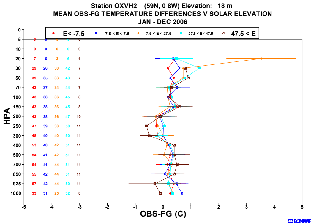
Figure 10 Temperature vertical statistics OB-FG (bias and STD) as a function of the solar elevation at the time of the observation. January to December 2006
